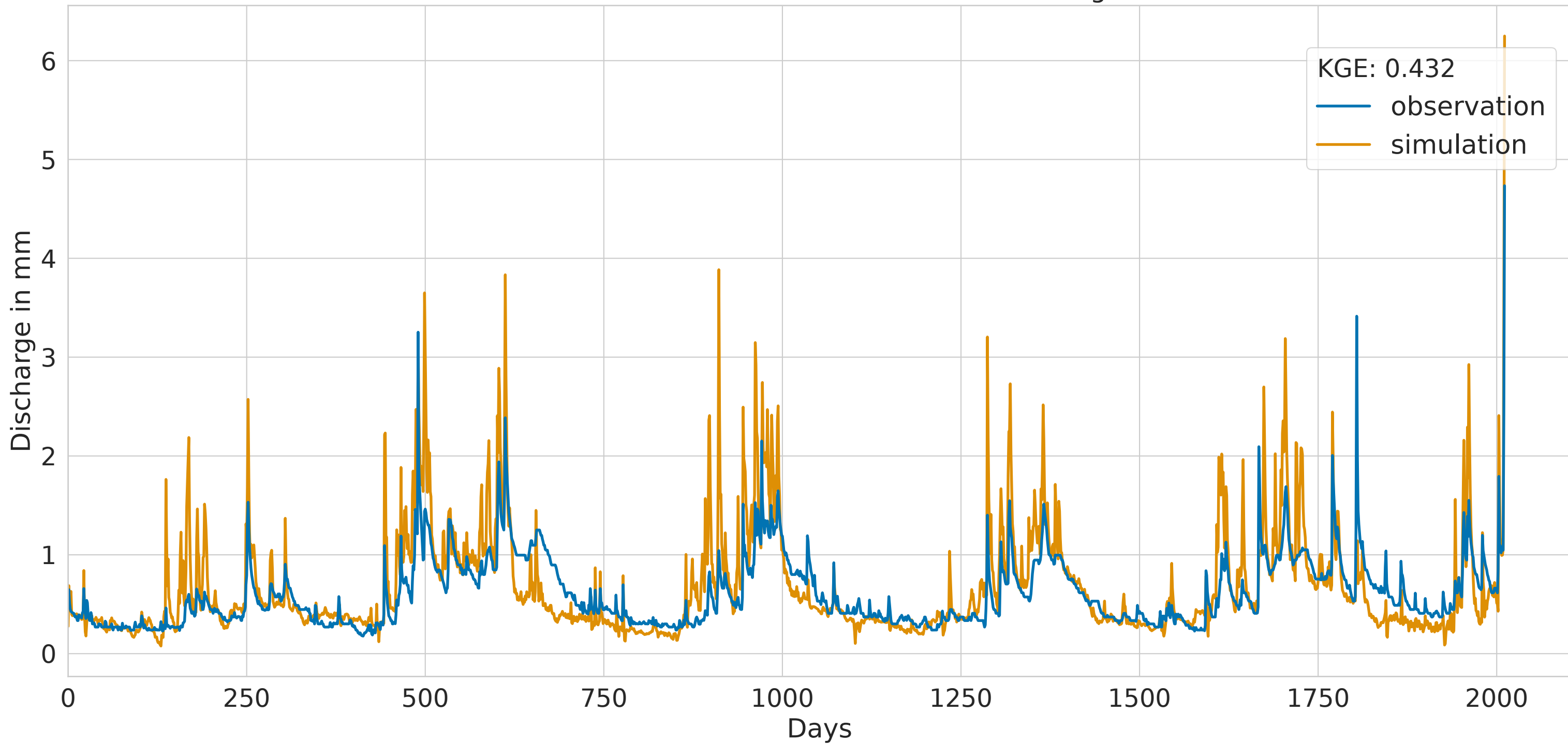
CNN with static features and batch size of 256 for Gauge 41860900
