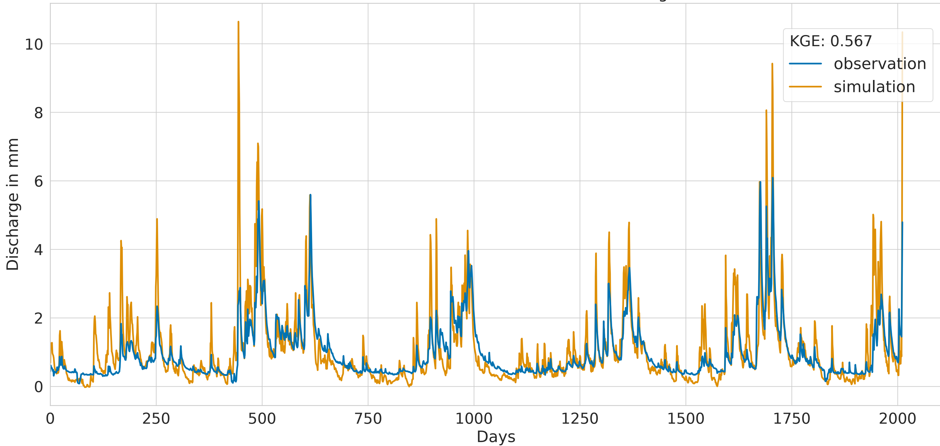
CNN with static features and batch size of 256 for Gauge 41510205
