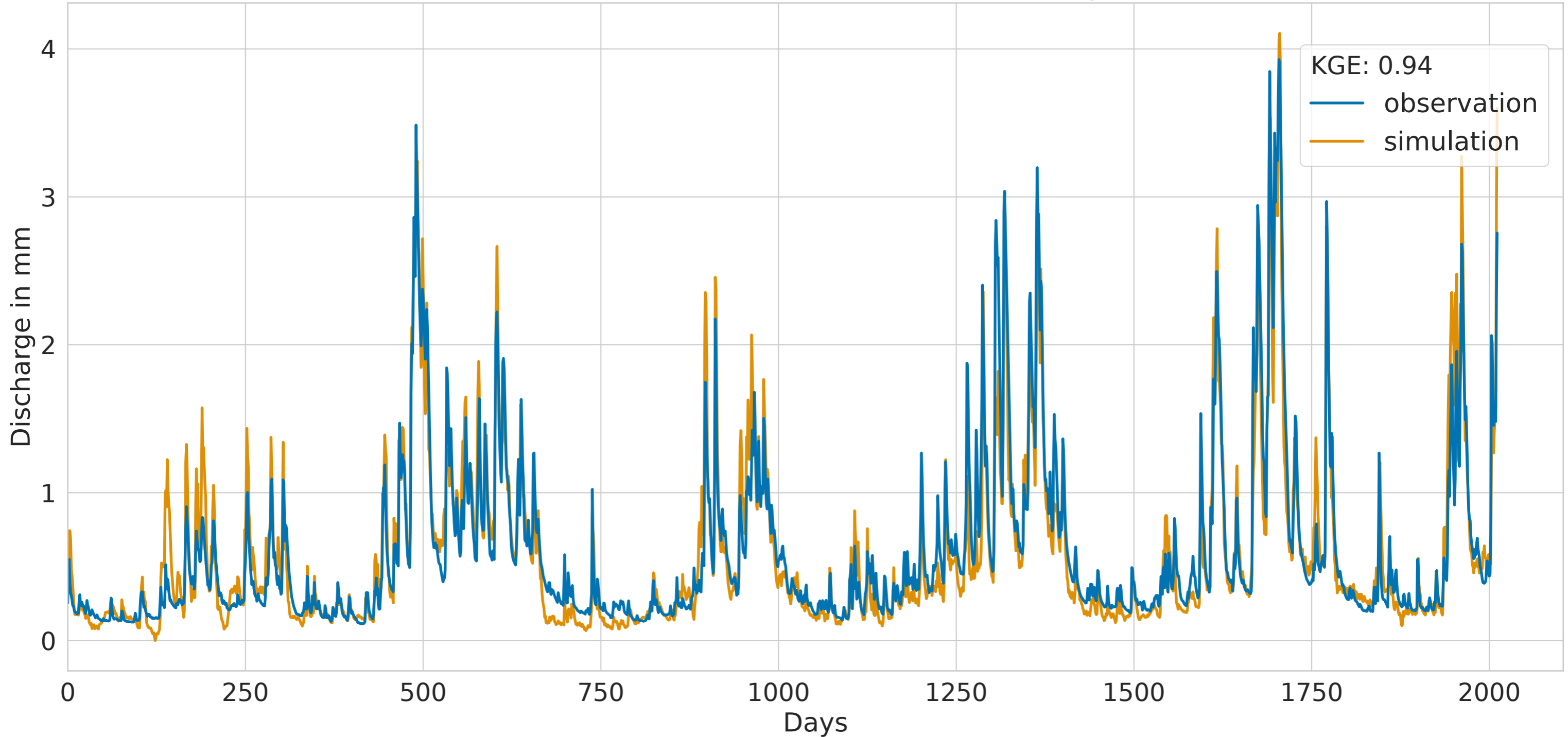
CNN with static features and batch size of 256 for Gauge 24870055
