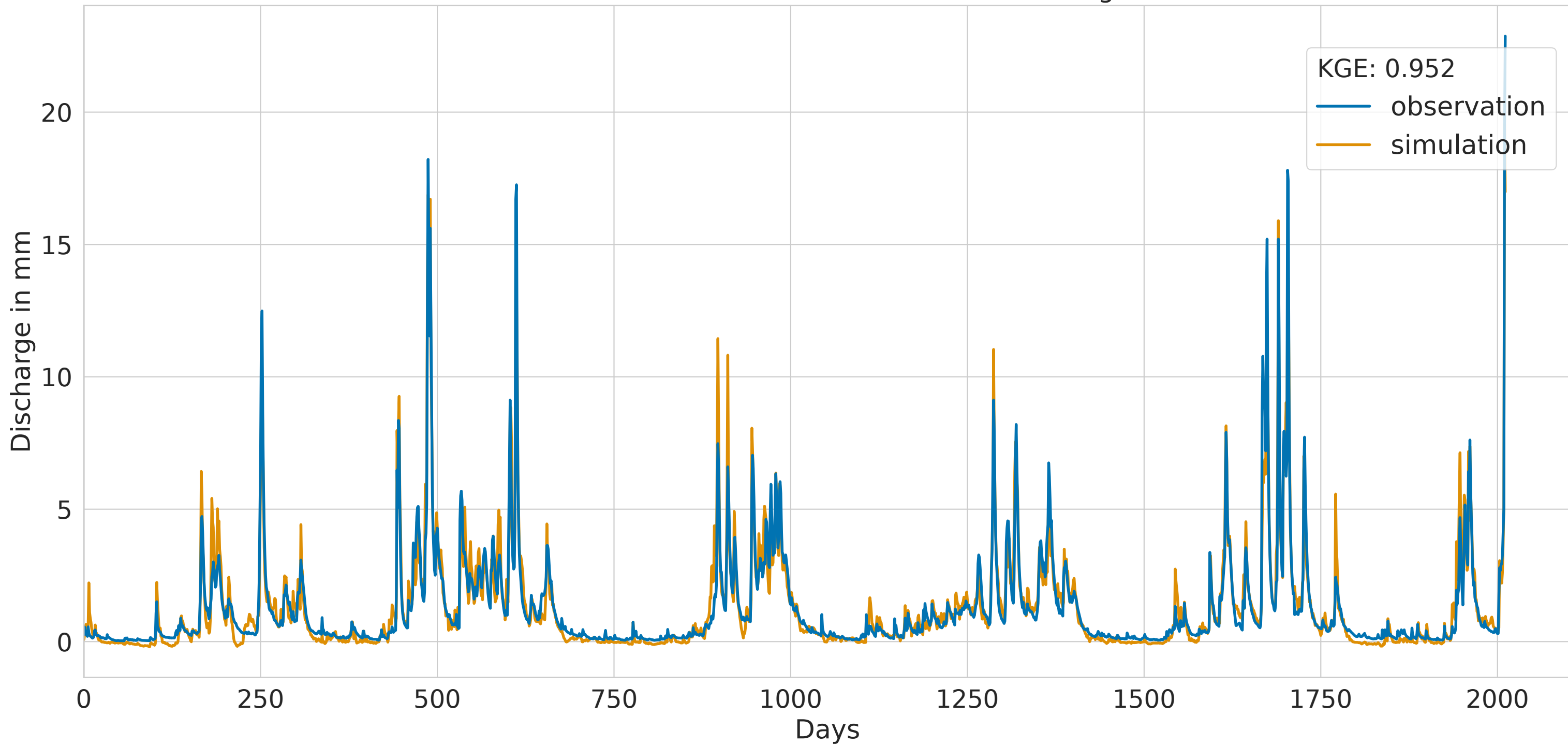
CNN with static features and batch size of 256 for Gauge 25840253
