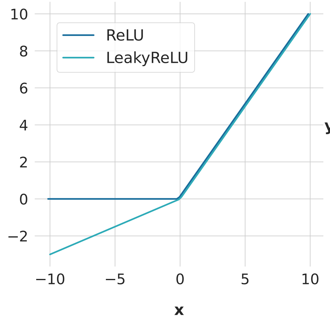
(b) ReLU Activation Functions
