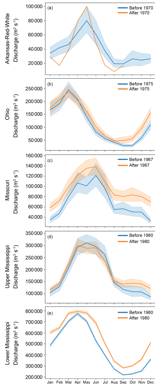
Figure A1. Mean monthly discharge values before and after periods of significant dam construction and river engineering for the tributaries (a) Arkansas-Red-White, (b) Ohio, (c) Missouri, (d) Upper Mississippi, (e) Lower Mississippi. Shading represents a 95 % confidence interval from interannual variability.
