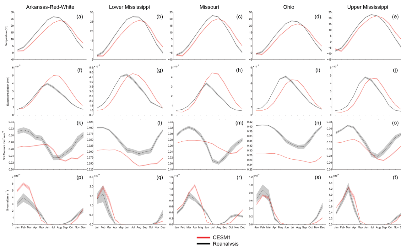
Figure A3. Monthly mean CESM1 simulated (red) values compared to reanalysis (black) values for temperature (a–e), evapotranspiration (f–j), soil moisture (k–o), and snowmelt (p–t) for the major subbasins: Arkansas-Red-White, Lower Mississippi, Missouri, Ohio, Upper Mississippi. Shading represents a 95 % confidence interval from ensemble spread for CESM1 data (50 ensemble members) and interannual variability for both CESM1 and reanalysis data.
