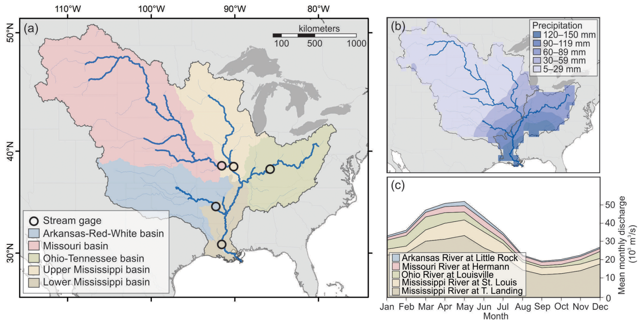
Figure 1. Mississippi River Basin and major tributaries: (a) Basins of major tributaries and corresponding stream gage locations. (b) Monthly mean (mm per month) precipitation from Global Precipitation Climatology Center (GPCC) 10 and grouping of subbasins into Eastern and Western Basins (gray line). (c) Monthly mean discharge from stream gages on the major tributaries (1950–2010).
