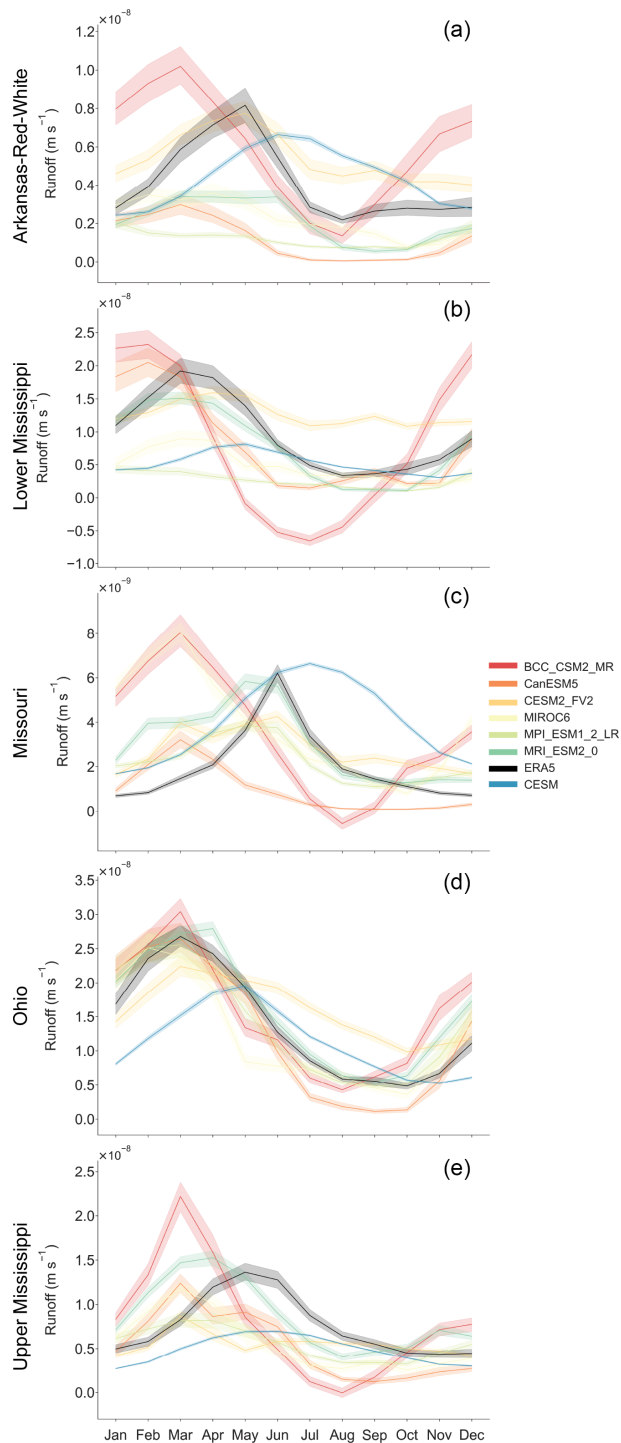
Figure A4. Monthly mean simulated runoff ( \text{m s}^{-1} ) from selected CMIP6 models (BCC CSM2 MR [red], CanESM5 [dark orange], CESM2 [light orange], MIROC6 [yellow], MPI ESM1 2 LR [light green], MRI ESM2 0 [dark green]), CESM1 [blue], and ERA5 re-analysis [black] for the Arkansas-Red-White (a), Lower Mississippi (b), Missouri (c), Ohio (d), and Upper Mississippi (e) basins. Shading represents a 95 % confidence interval from interannual variability.
