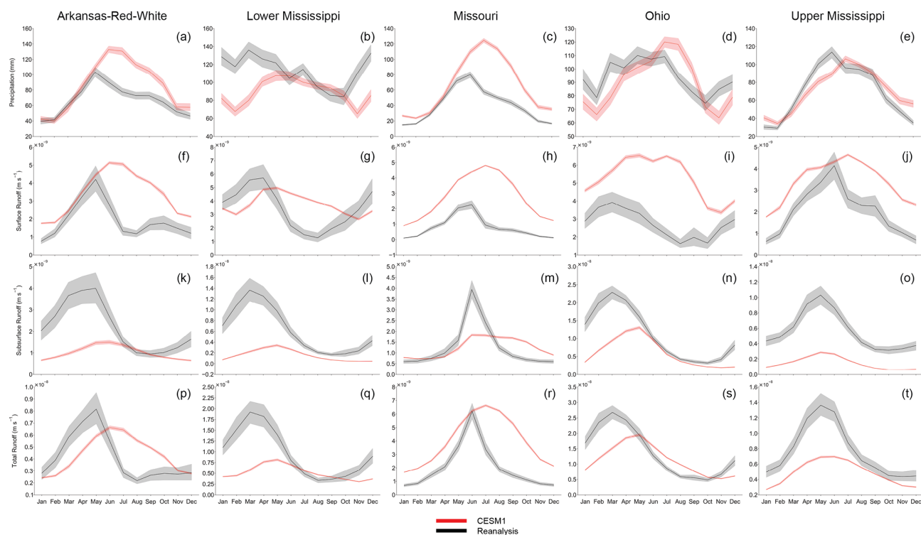
Figure A2. Monthly mean CESM1 simulated (red) values compared to reanalysis (black) values for precipitation (a–e), surface runoff (f–j), subsurface runoff (k–o), and runoff (p–t) for the major subbasins: Arkansas-Red-White, Lower Mississippi, Missouri, Ohio, Upper Mississippi. Shading represents a 95 % confidence interval from ensemble spread for CESM1 data (50 ensemble members) and interannual variability for both CESM1 and reanalysis data.
