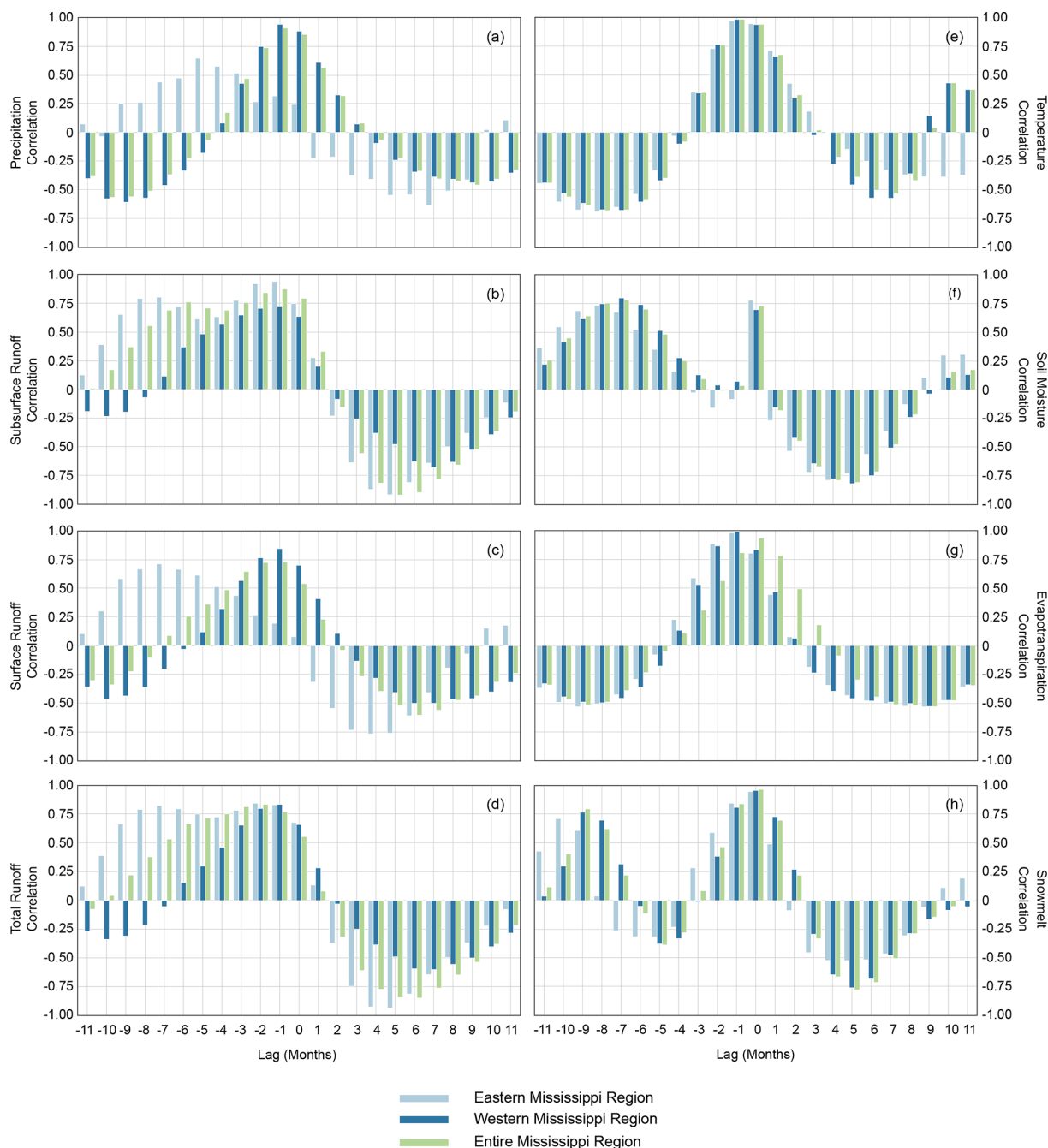
Figure 5. Monthly lag correlation values for each hydrologic variable: (a) precipitation, (b) subsurface runoff, (c) surface runoff, (d) runoff, (e) temperature, (f) soil moisture, (g) ET, (h) snowmelt, for each region: Eastern Mississippi basin (light blue), Western Mississippi Basin (dark blue), Entire Mississippi basin (green).
