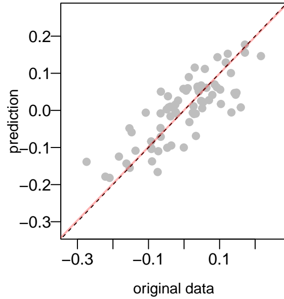
Cross-validation: r = 0.81
