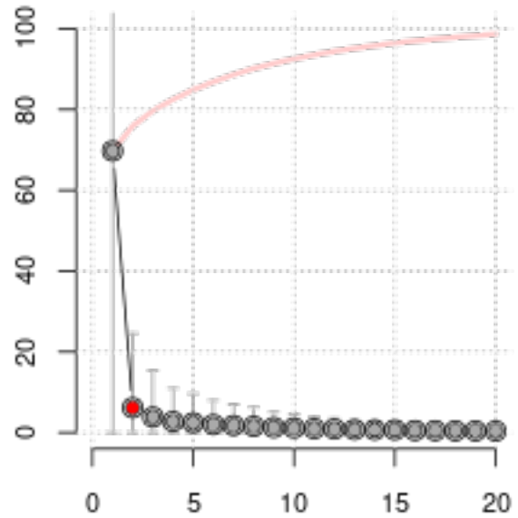
20 leading EOFs: 98.7 % of variance
