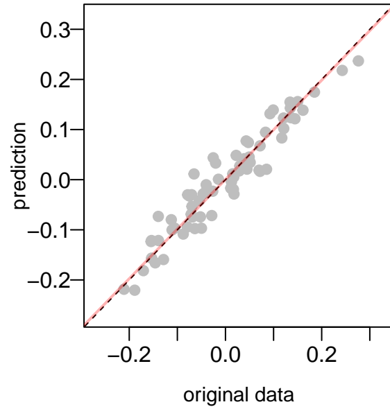
Cross-validation: r = 0.96
