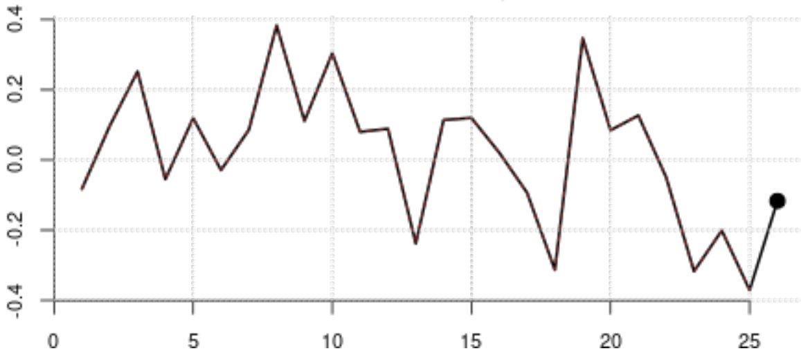
Leading PC#2 of trend coefficients - Explained variance = 6.15%
