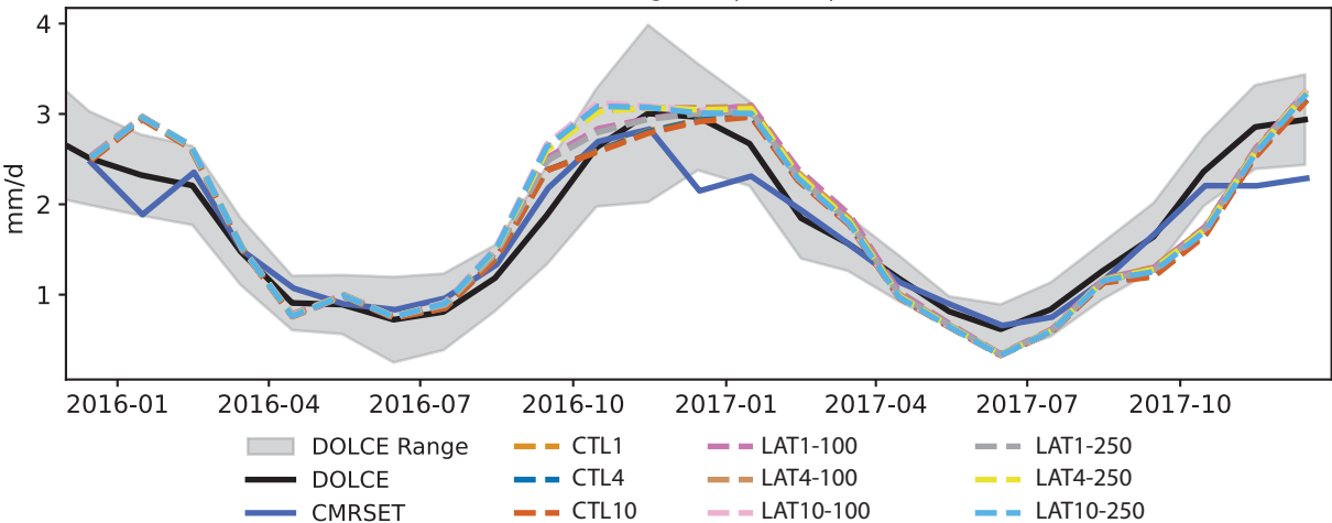
Domain Average Evapotranspiration
