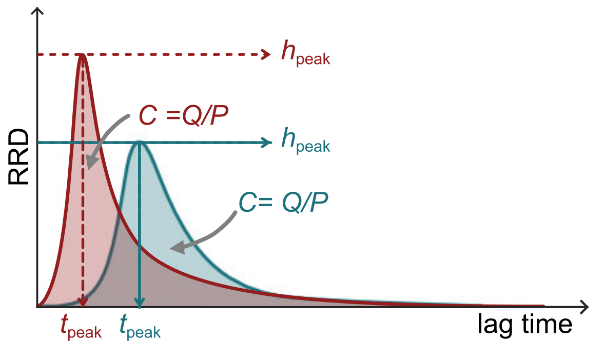
(c) Runoff response distributions (RRD)
