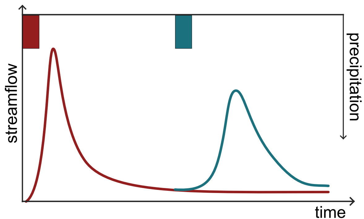
(a) Hydrologic response
