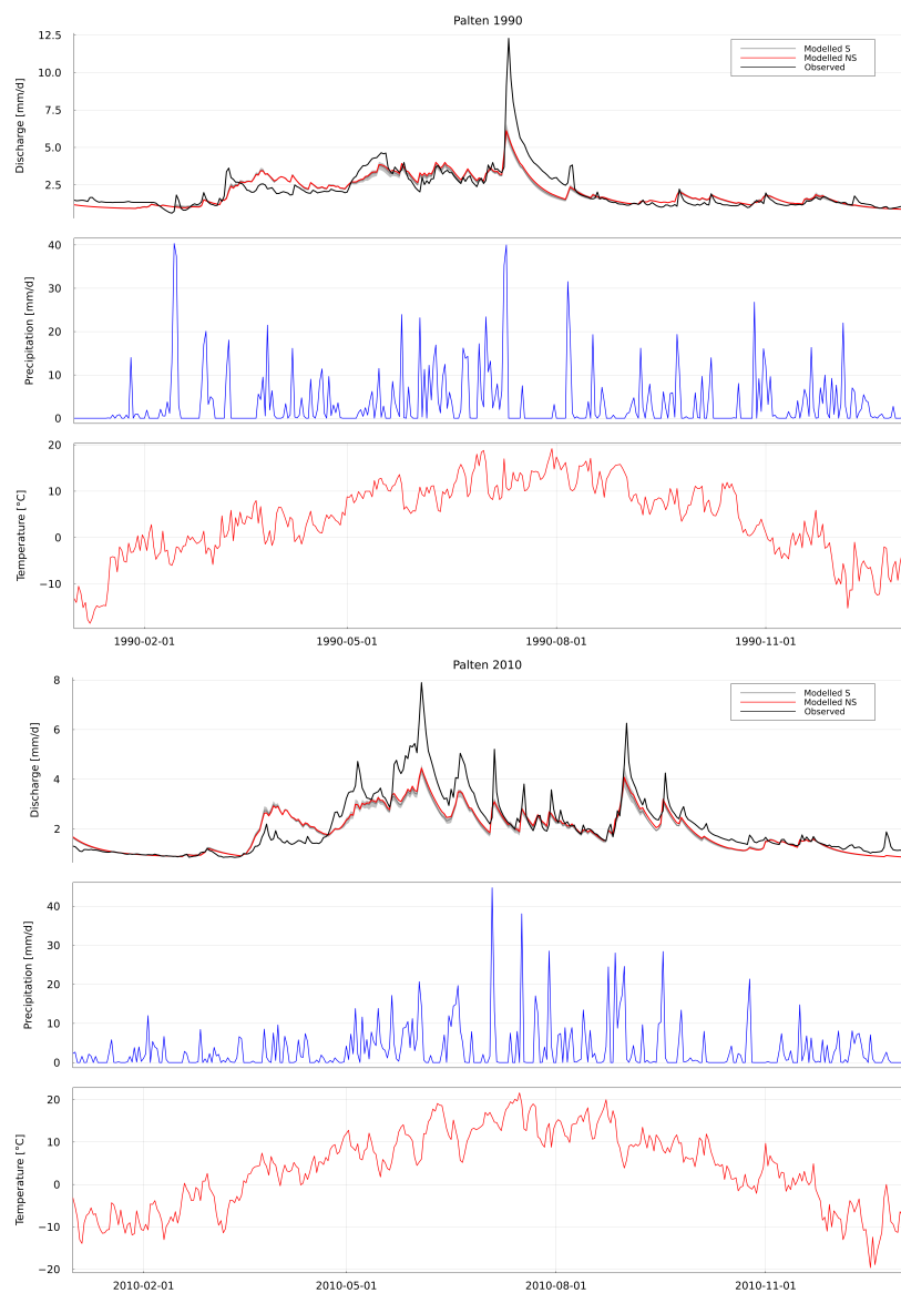
Fig. S 10. Comparison of measured and both calibrated and climate-based modelled runoff in the Paltental, also showing the corresponding temperature and precipitation. The solid lines indicate mean modelled runoff using the best parameter sets, shaded areas show the range of best parameter sets
