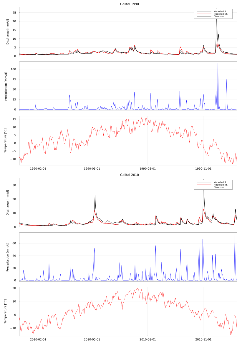
Fig. S9. Comparison of measured and both calibrated and climate-based modelled runoff in the Gaital, also showing the corresponding temperature and precipitation. The solid lines indicate mean modelled runoff using the best parameter sets, shaded areas show the range of best parameter sets
