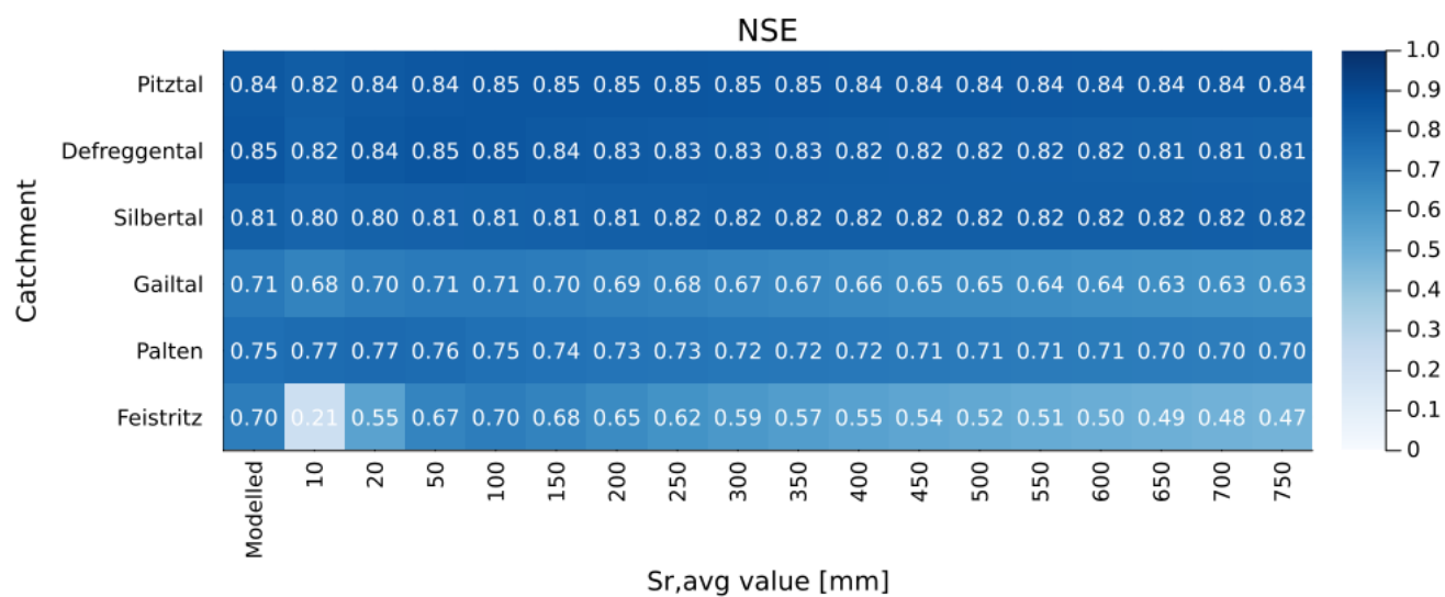
Fig. S 17. Sensitivity analysis of the HBV model during the sensitivity period (Pitztal: 1985–2007; Gailtal: 1985–2010; other catchments: 1985–2012). The heatmap shows relative model performance (NSE) for varying average S_R values and catchment-average storage capacities, averaged across vegetation types.
