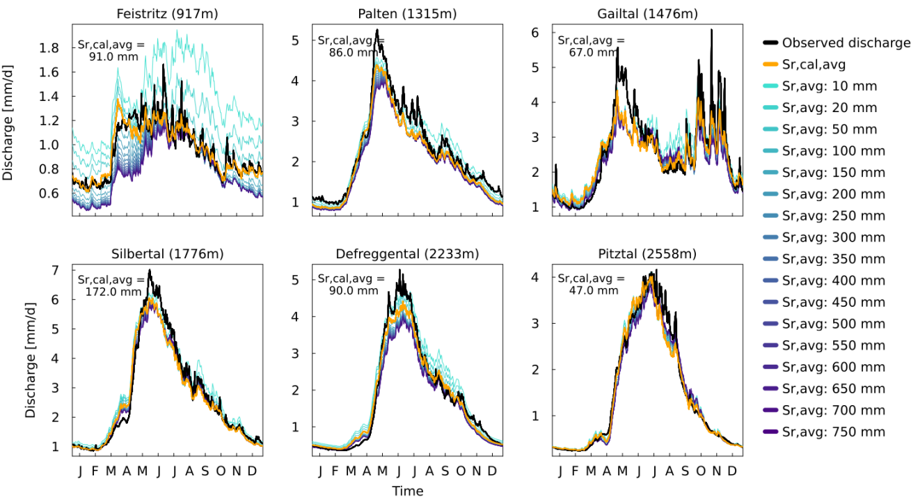
Fig. S 16. Sensitivity analysis of the HBV model during the sensitivity period (Pitztal: 1985–2007; Gailtal: 1985–2010; other catchments: 1985–2012). The plots show observed discharge and mean regime curves for different catchment-average storage capacities, averaged across vegetation types.
