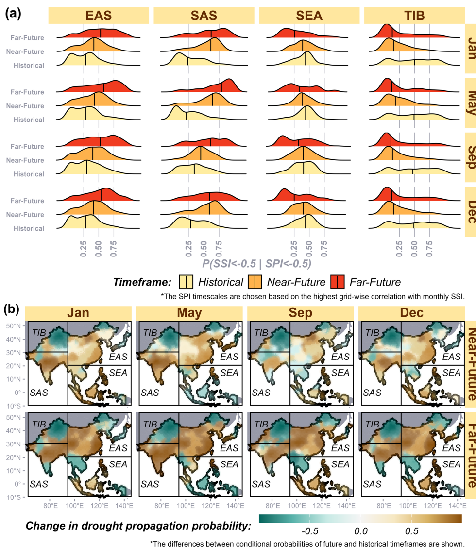
Figure 4. (a) Comparison of propagation probabilities across four regions, seasons, and time frames and (b) spatial maps showing the differences in propagation probabilities between future and historical time frames.
