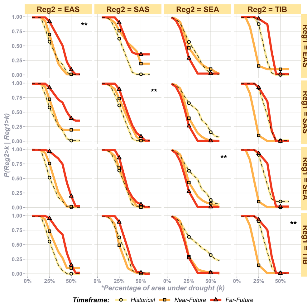
Figure 10. Probability of a region exceeding different values of drought spatial coverage ( k ), which is conditioned on similar spatial coverage in another region, compared across time frames.
