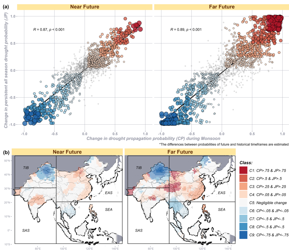
Figure 12. (a) Relationship between drought propagation and persistence using changes in their probability values in the future and historical time frames and (b) spatial maps showing bivariate classification based on future persistence and propagation values to identify vulnerable grids.
