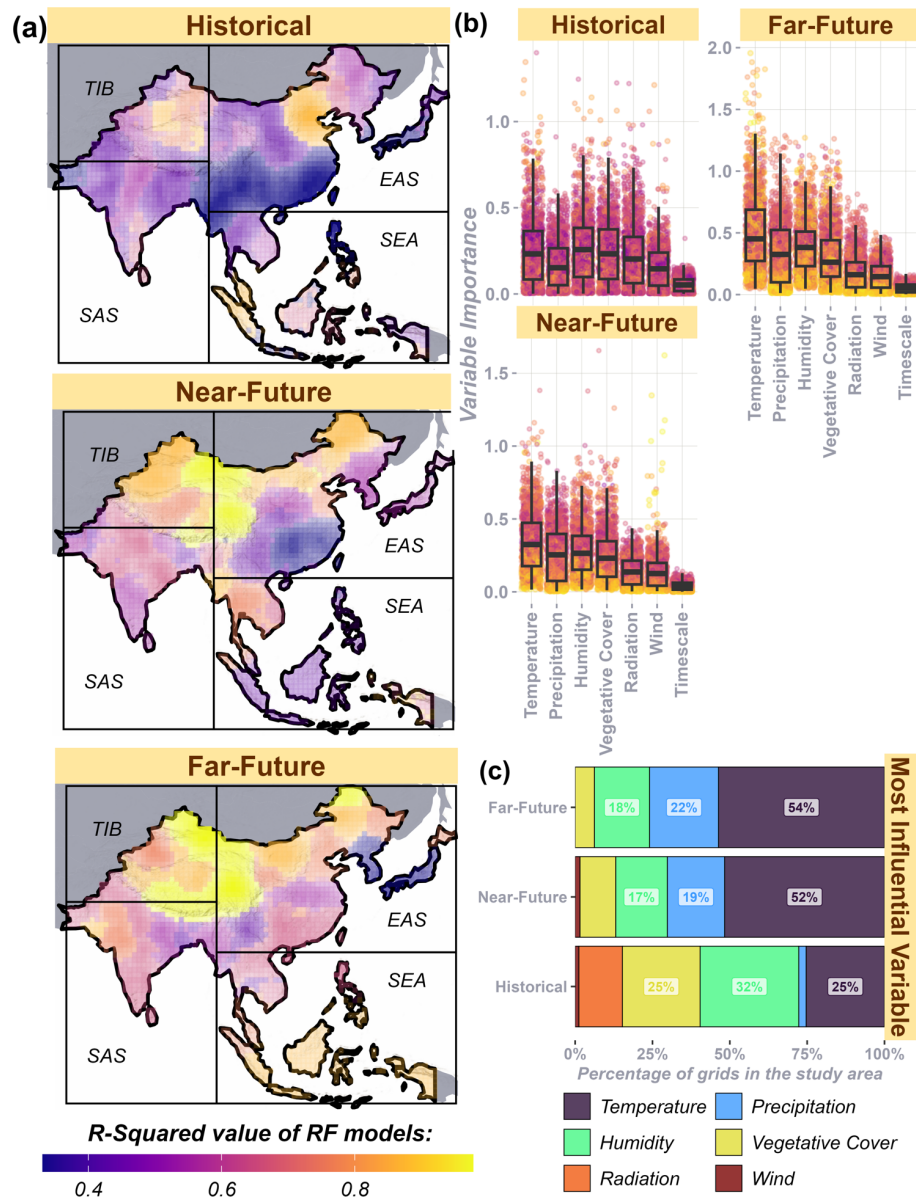
Figure 5. (a) Performance evaluation ( R^2 values) of random forest (RF) models for each grid across time frames, (b) variable importance values of predictors used in the RF models, and (c) the most important variable (highest importance value in an RF model) in each time frame across the study area.
