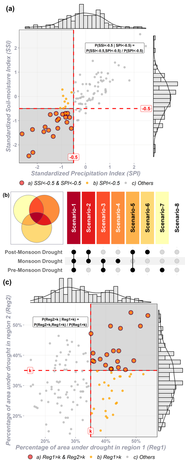
Figure 1. (a) Domain of the conditional probability defining the propagation from meteorological to agricultural drought, (b) Venn diagram of all possible inter-seasonal drought scenarios, and (c) domain of conditional and joint exceedance probability for studying drought spatial concurrence.
