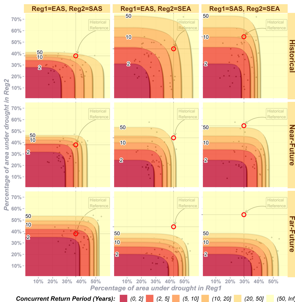
Figure 11. Spatial concurrent return periods between region pairs across time frames, with random variables (the percentage of area under drought annually) shown as black dots.
