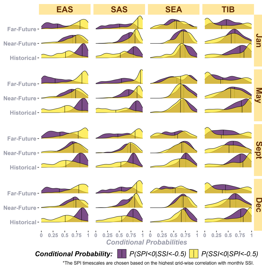
Figure 7. The reverse-propagation probability ( P(SPI < 0 | SSI < -0.5) ) indicates if an agricultural drought is linked to a prior meteorological drought.
