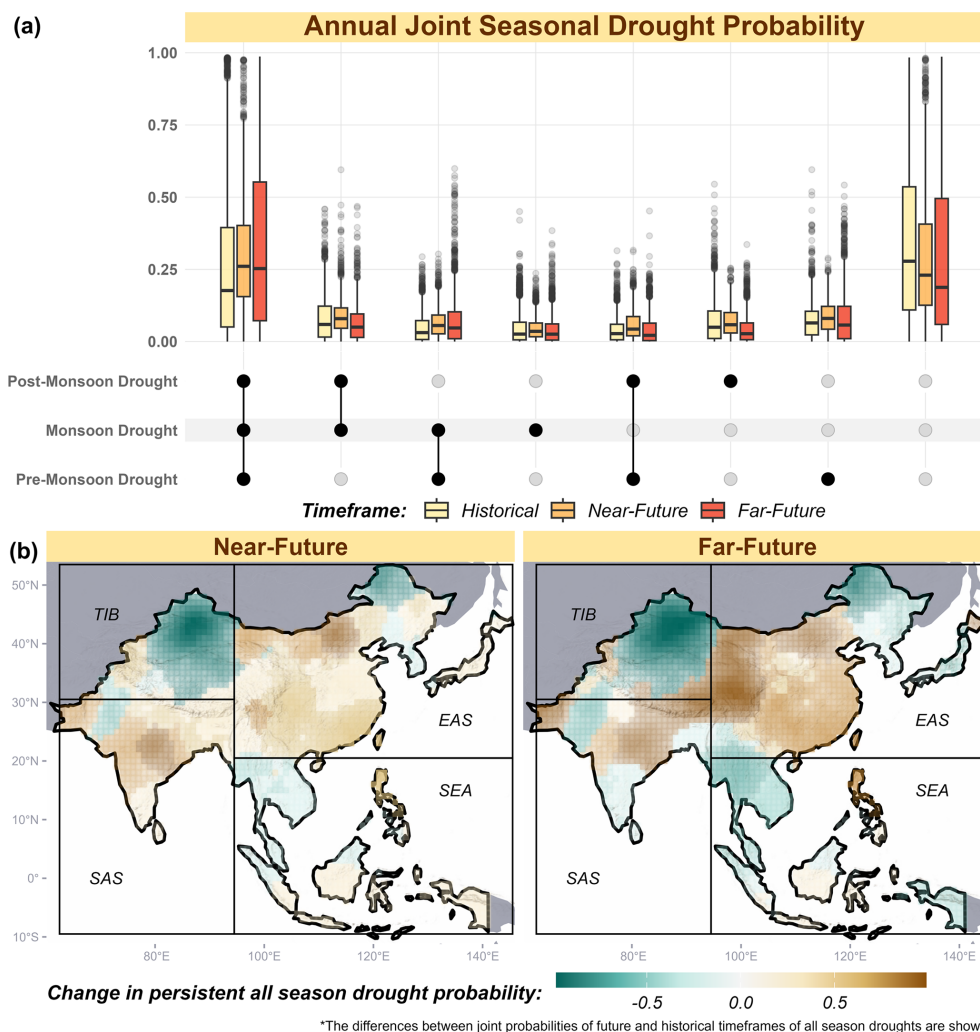
Figure 8. (a) Joint probabilities of all inter-seasonal drought scenarios across the study area for three time frames and (b) maps showing differences in all-season drought probabilities between future and historical time frames.
