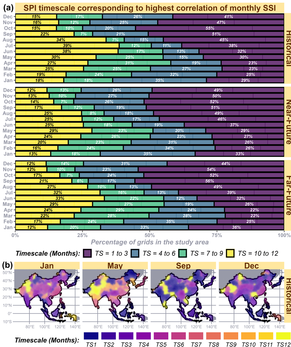
Figure 3. Propagation durations (in timescale, TS) shown as (a) percentages across the study area for each month in different time frames and (b) spatial maps for different seasons in the historical time frame.
