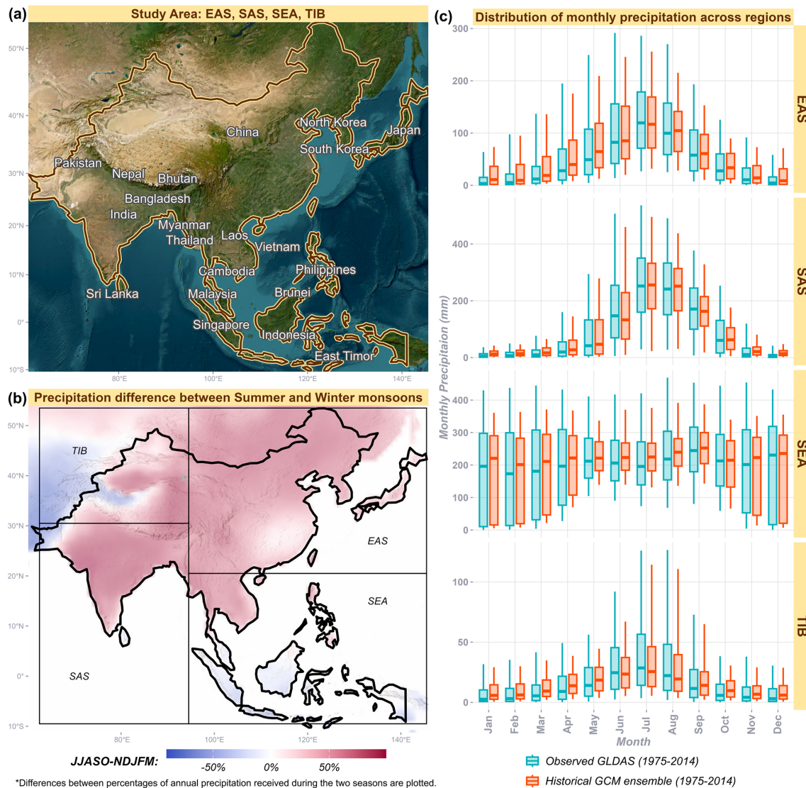
Figure 2. (a) Study area of monsoon-dominant Asia with its boundaries (geographic information system, GIS, base map layers were downloaded from Esri et al. (2025) and administrative boundary shapefiles from Natural Earth (2025)); (b) percentage difference in precipitation between summer (June–October) and winter (November–March) monsoons, regional divisions are based on thematic maps from works such as Giorgi and Bi (2009) and Sillmann et al. (2013); and (c) a monthly comparison of observed and historical GCM precipitation data across the four regions.
