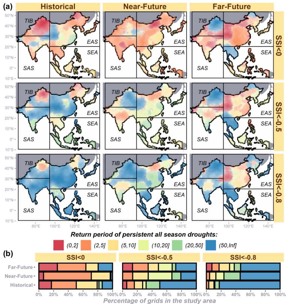
Figure 9. Return periods of persistent all-season droughts for various agricultural drought severity levels across time frames, shown as (a) maps and (b) percentages of the study area.
