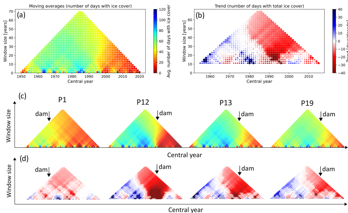
Figure 6. Moving average (a) and trend (b) charts showing the number of days with ice cover created from averages of reservoir-influenced water gauges. Panels (c) and (d) show MARTA graphs created using data from individual water gauges.
