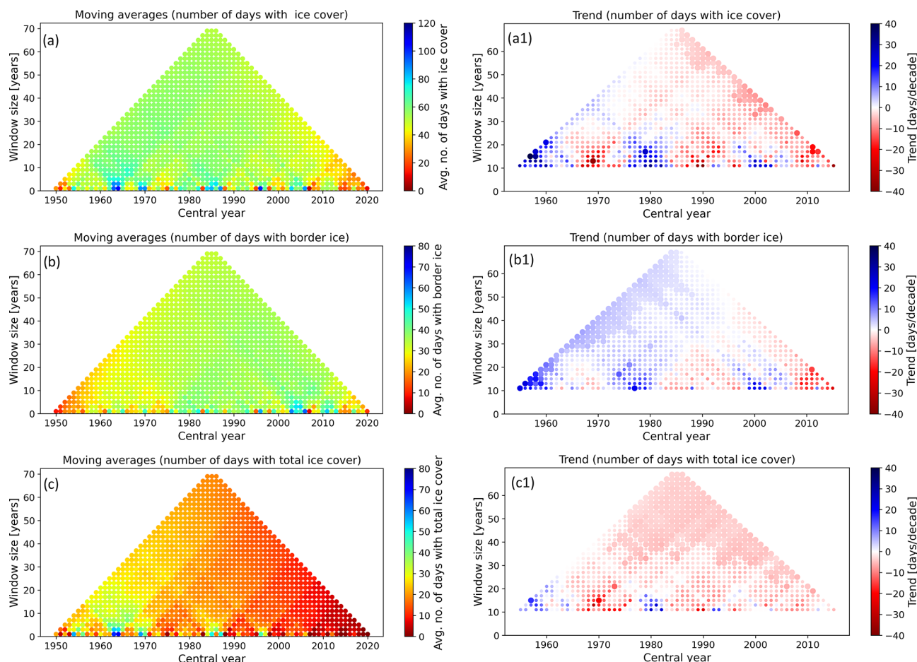
Figure 2. MARTA triangles showing the moving average (a–c) and trend (number of days per decade; a1, b1, and c1) in the average annual number of days (using average values from all P1–P25 stations) with border ice (b and b1), total ice cover (c and c1), and the sum of these phenomena (a and a1). In the graphs of (a1), (b1), and (c1), statistically significant values at the p < 0.05 level are marked with larger markers.
