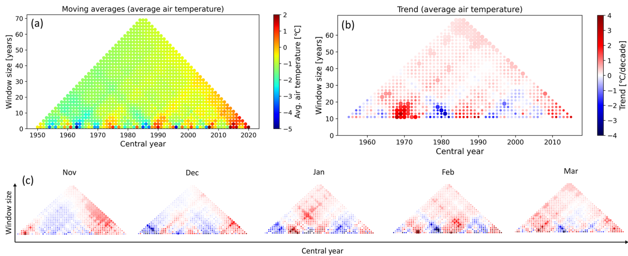
Figure 5. MARTA graphs showing the moving averages (a) and trend (b) in the average air temperature of the winter period and individual months (c) for the period 1950–2020. In graphs (b) and (c), statistically significant values at the p < 0.05 level are marked with larger markers.
