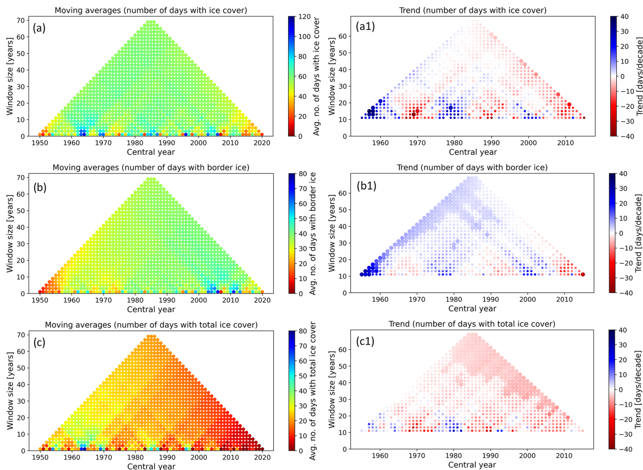
Figure 4. MARTA graphs showing the moving average (a–c) and trend (number of days per decade; a1, b1, and c1) in the average annual number of days at stations (average values from non-human-influenced water gauges) with border ice (b and b1), total ice cover (c and c1), and the sum of these phenomena (a and a1). In graphs (a1), (b1), and (c1), statistically significant values at the p < 0.05 level are marked with larger markers.
