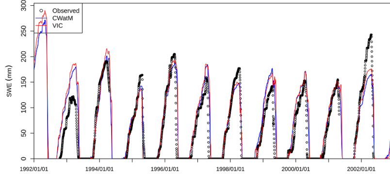
Figure S1. Observed vs. simulated SWE from CWatM and VIC models for three stations with highest numbers of observations.
