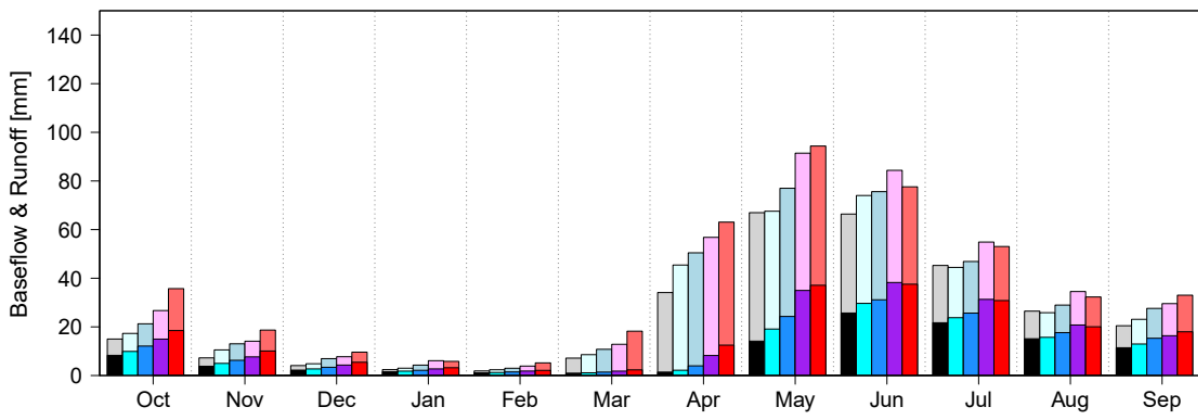
Figure S2. Sample annual and monthly runoff distribution obtained from CanESM5 GCM driven VIC and CWatM runs for historical (1971-2000) and 1.5 to 4.0 °C GWLs. The upper and lower portions of the bar plots show surface runoff and baseflow, respectively.
