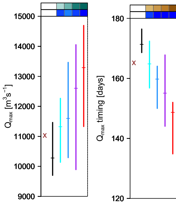
(a) Liard-M: VIC
