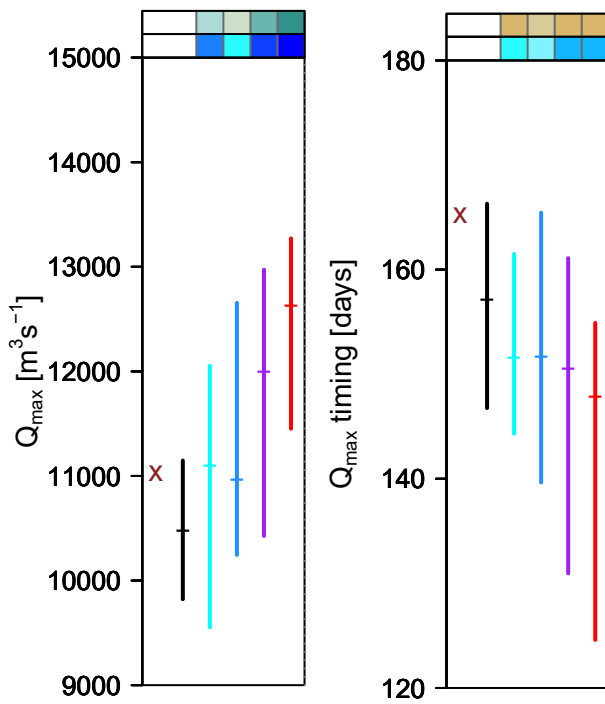
(b) Liard-M: CWatM
