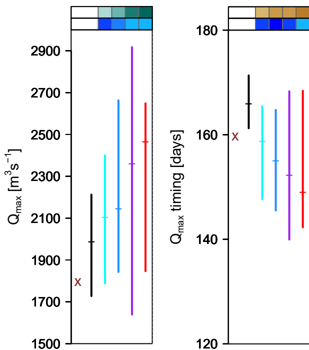
(c) Liard-UC: VIC
