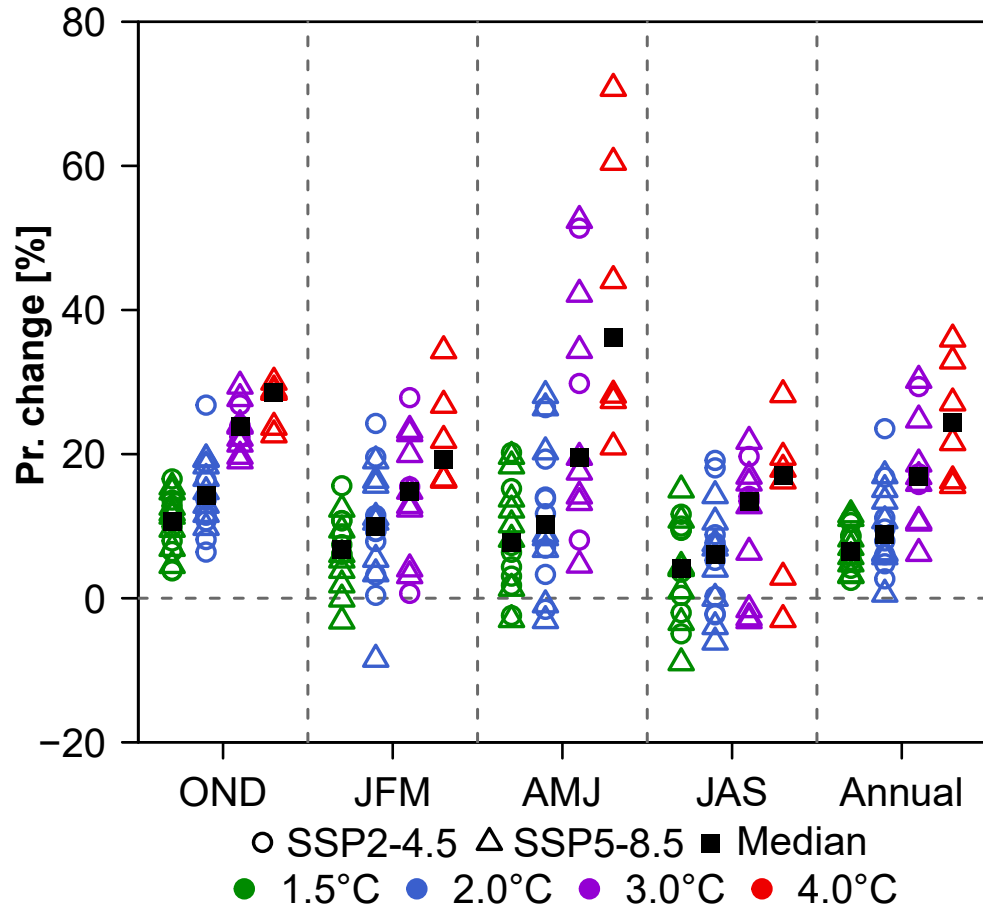
(b) Mean precipitation
