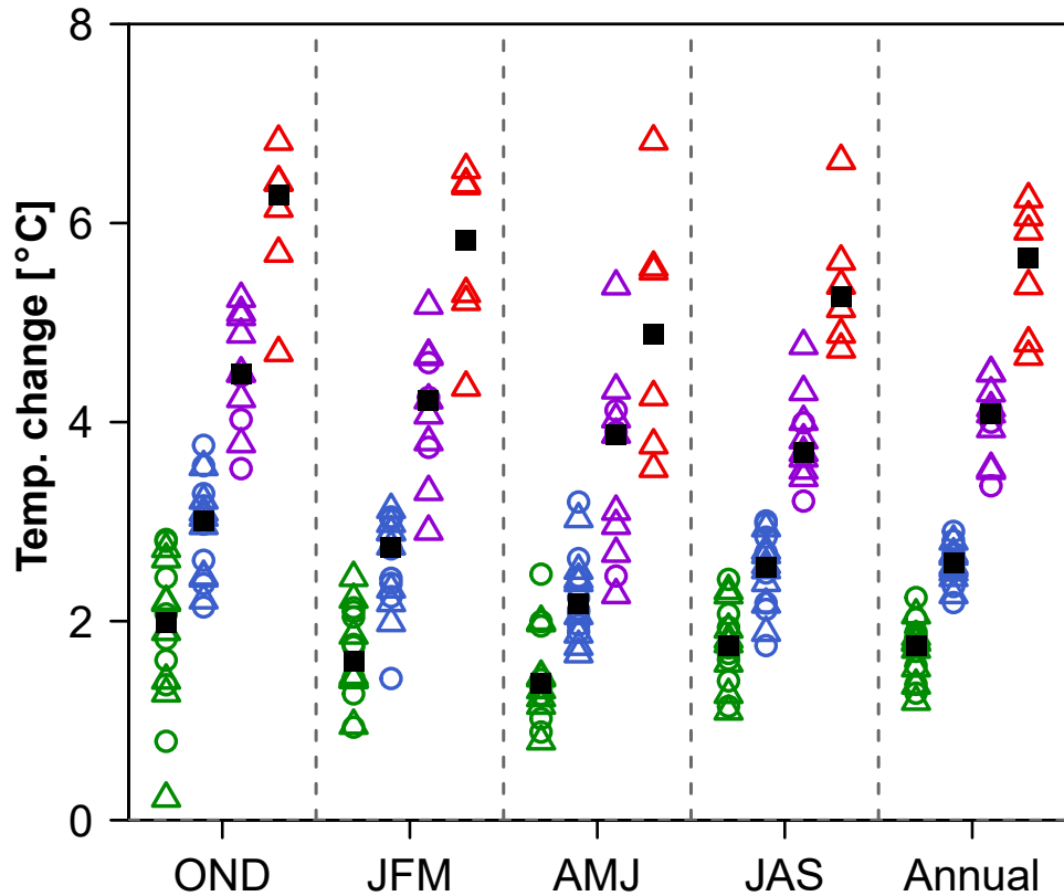
(a) Mean temperature
