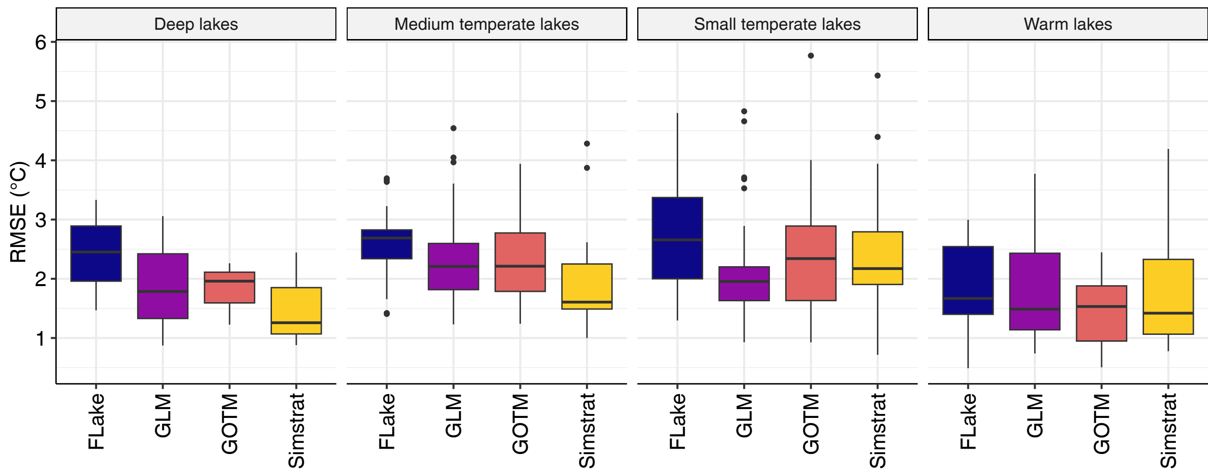
(b) RMSE at thermocline depth
