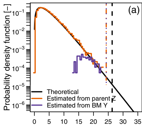
Sample size: 100 years
