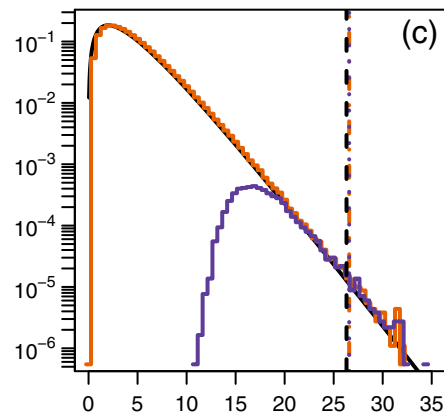
Sample size: 10000 years
