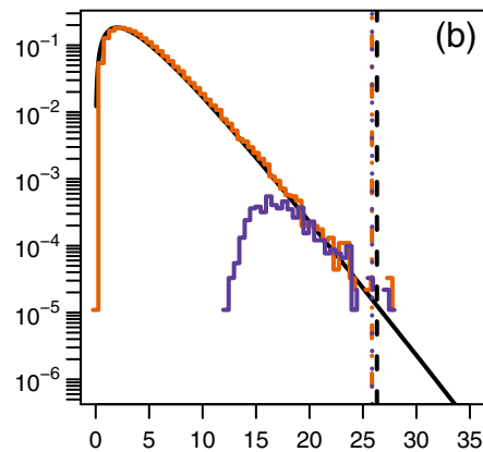
Sample size: 500 years
