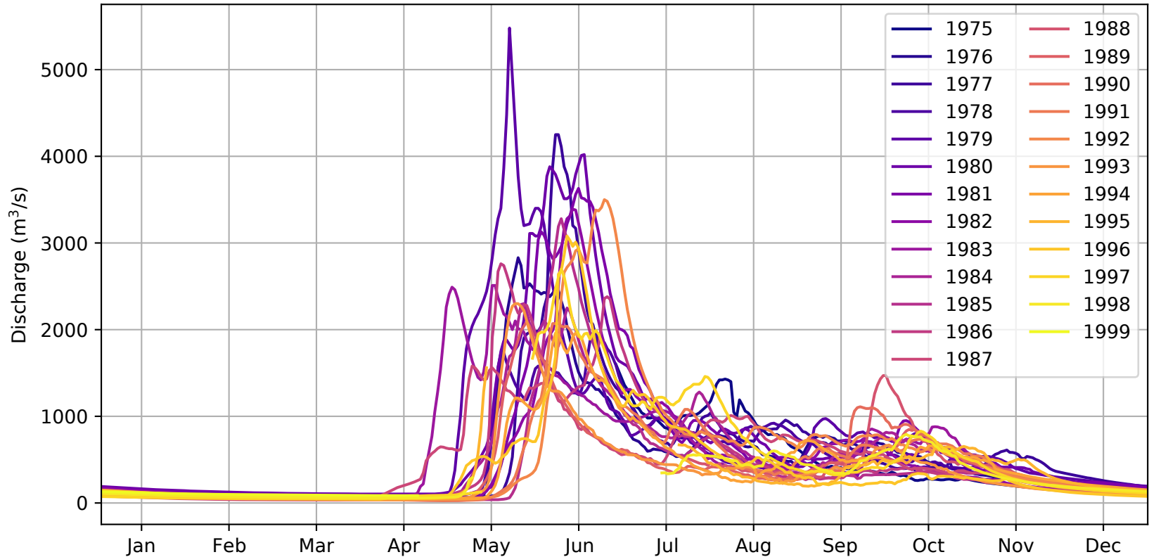
Yearly discharge at Lac de la Hutte Sauvage station from 1975 to 1999
