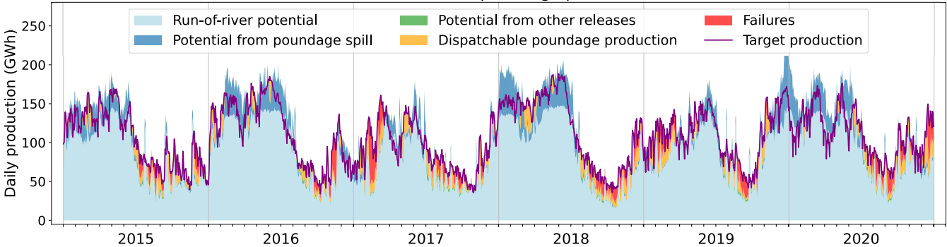
Run-of-river and poundage production
