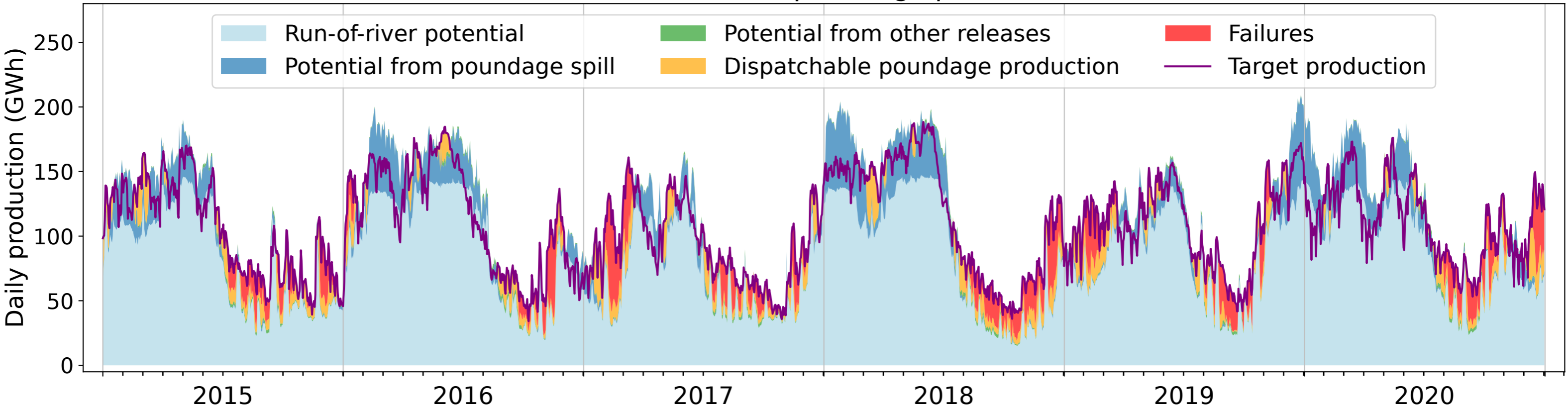
Run-of-river and poundage production
