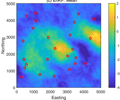
(c) EnKF: Mean
