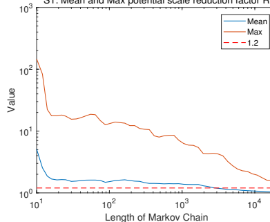
S3: Mean and Max potential scale reduction factor R
