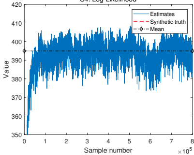
S4: Log-Likelihood
