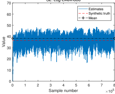
S2: Log-Likelihood
