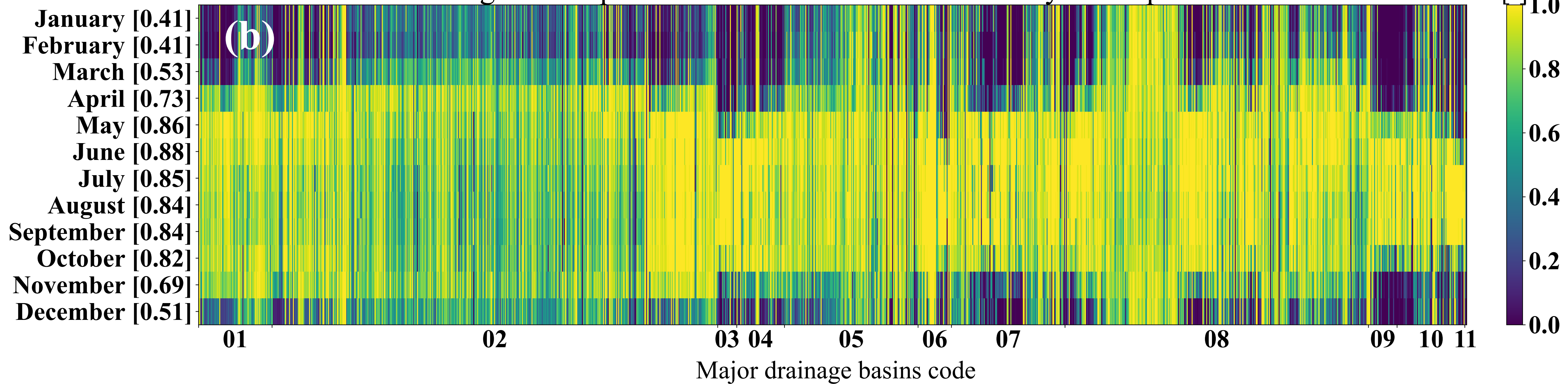
Fraction of reproducibility for reported discharge in the WSC database using the independent workflow within an accuracy of 5.0 percent
