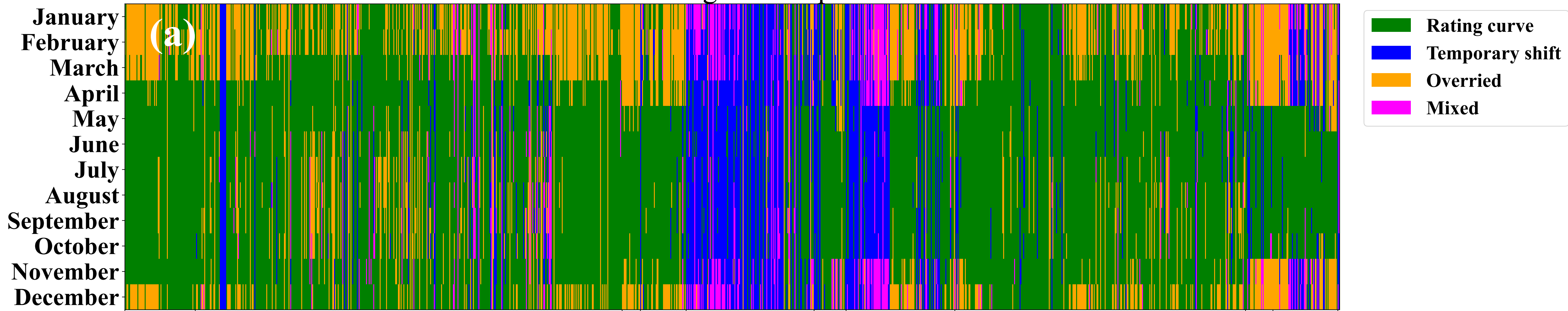
Fraction of reproducibility for reported discharge in the WSC database using the independent workflow within an accuracy of 5.0 percent
