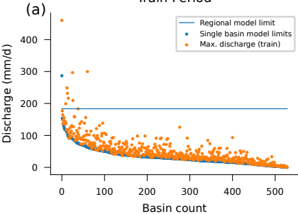
Train Period
