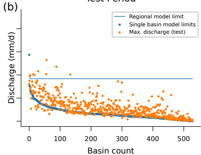
Test Period
