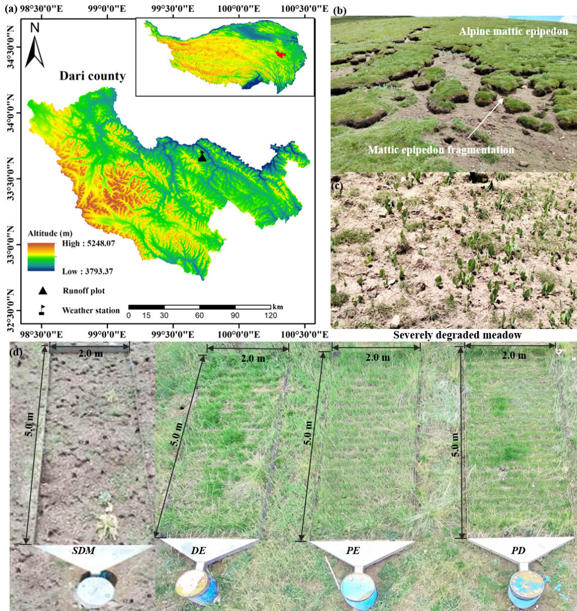
Figure 1. The location of the study area on the Qinghai–Tibetan Plateau and the locations of runoff plots in the study area. (a) The location of the study area, (b) the fragmenting matted epipedon on the alpine hillslope, (c) severely degraded meadow (SDM) formed by the disappearance of the matted epipedon, and (d) four runoff plots of SDM and mixed-cultivation grasslands. A typical severely degraded meadow with a slope of 20° was selected to plant mixed grasses. Runoff plots were photographed with a drone in the early stages of the 2022 growing season: DE – Deschampsia cespitosa and Elymus nutans ; PE – Poa pratensis L. cv. Qinghai and Elymus nutans ; and PD – Poa pratensis L. cv. Qinghai and Deschampsia cespitosa .
