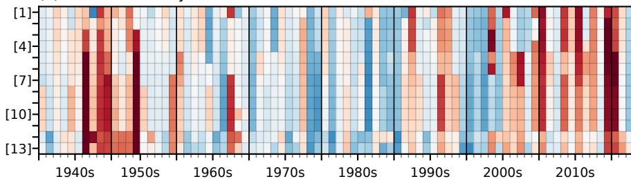
(c) Natural anomaly of wet season duration
