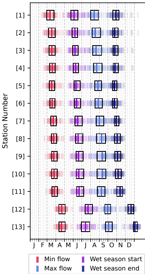
(a) Natural variation of seasonal timing
