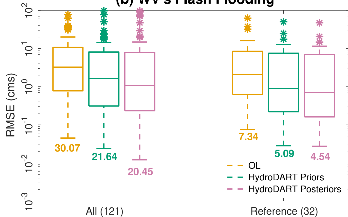
(b) WV's Flash Flooding
