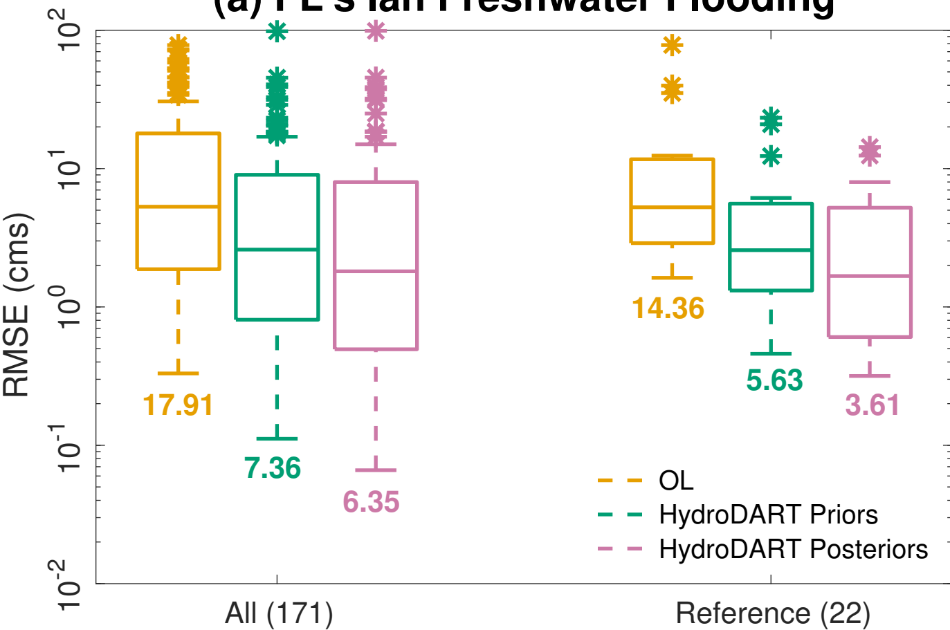
(a) FL's Ian Freshwater Flooding
