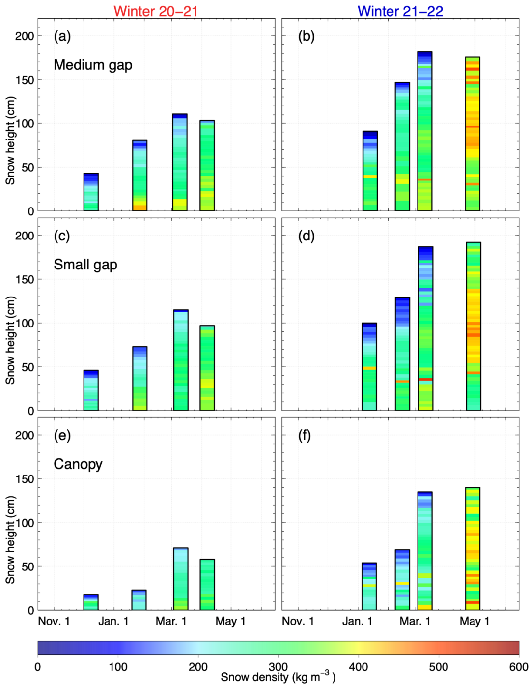
Figure S11: Snow density profiles from snow pit measurements in the medium and small gaps, and under the canopy during winters 2020–21 and 2021–22.
