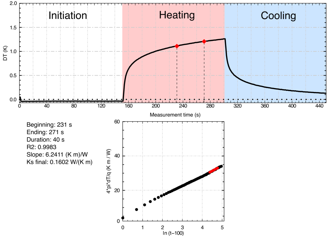
15 Figure S1: Heating curve analysis for the 80 cm needle from the monitoring station in the medium gap on 2 February 2022. In this example, we selected a period of 40 seconds that started at 231 seconds. The slope is 6.24 K m W -1 which gives a k_s of 0.16 W m -1 K -1 . Since R^2 is greater than 0.98 and no convection was detected, the measurement is considered valid.
