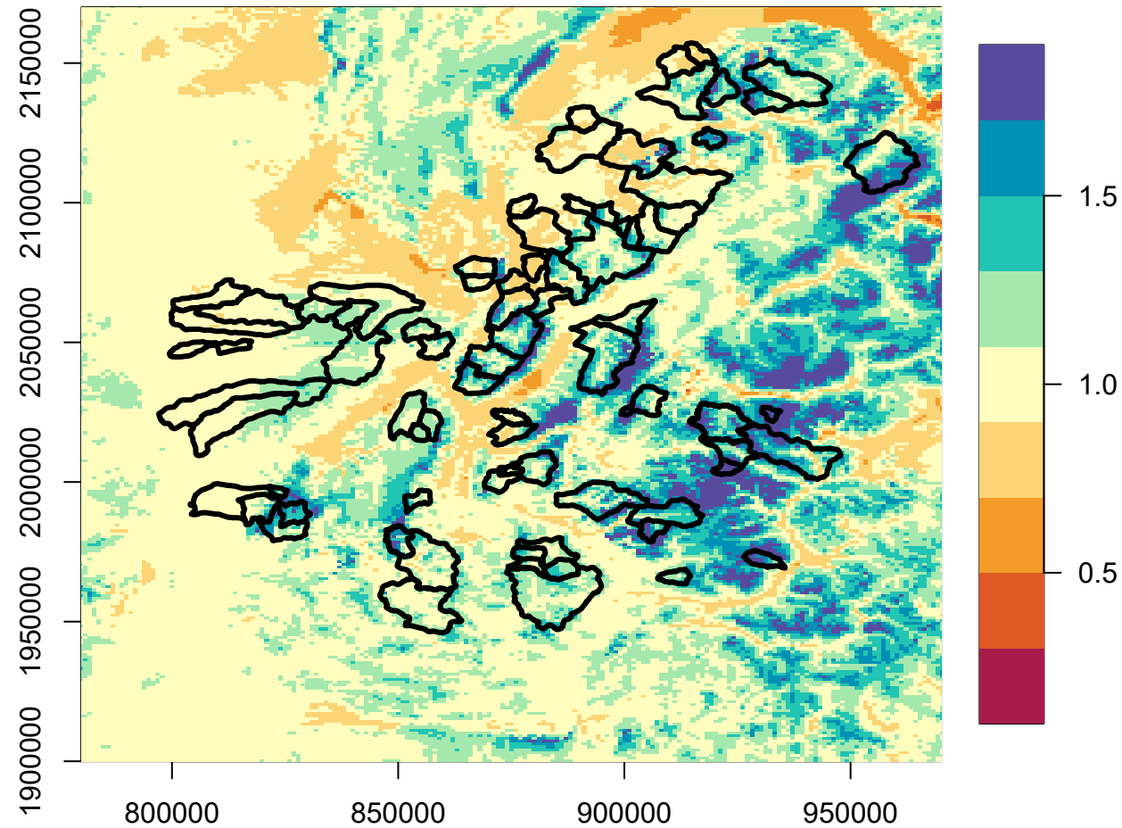
(a) Ratio SPAZM/COMEPHORE of mean annual Prec.
