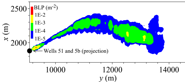
(g) Overlap of (c) and (f)
