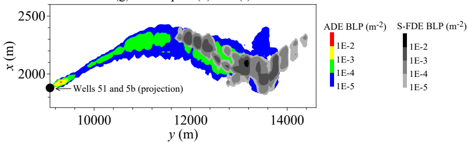
(g) Overlap of (c) and (f)
