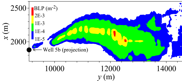
(f) Adjoint ADE: Joint BLP for Wells 51 and 5b, np=1000000
