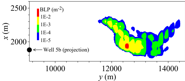
(c) Adjoint S-FDE: Joint BLP for Wells 51 and 5b, np=1000000
