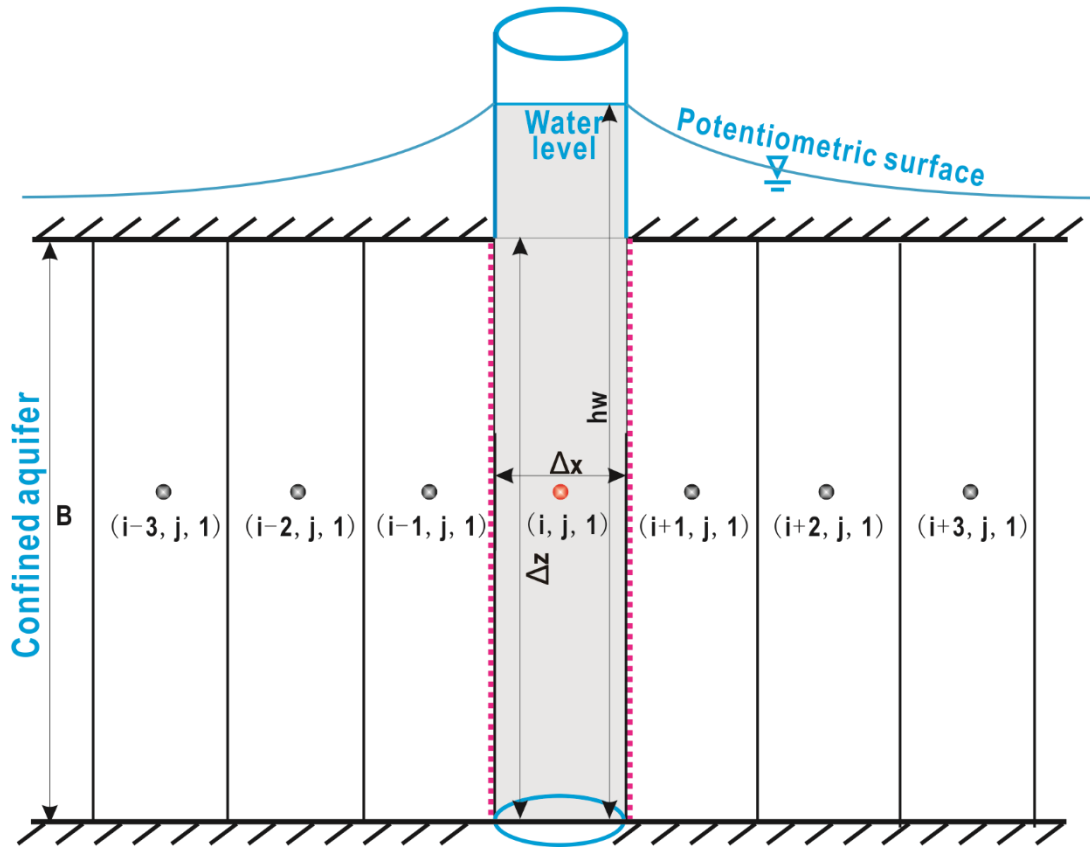
Figure S1. A cross section of 2D grid system of reactive transport model in a wellbore-confined aquifer system
