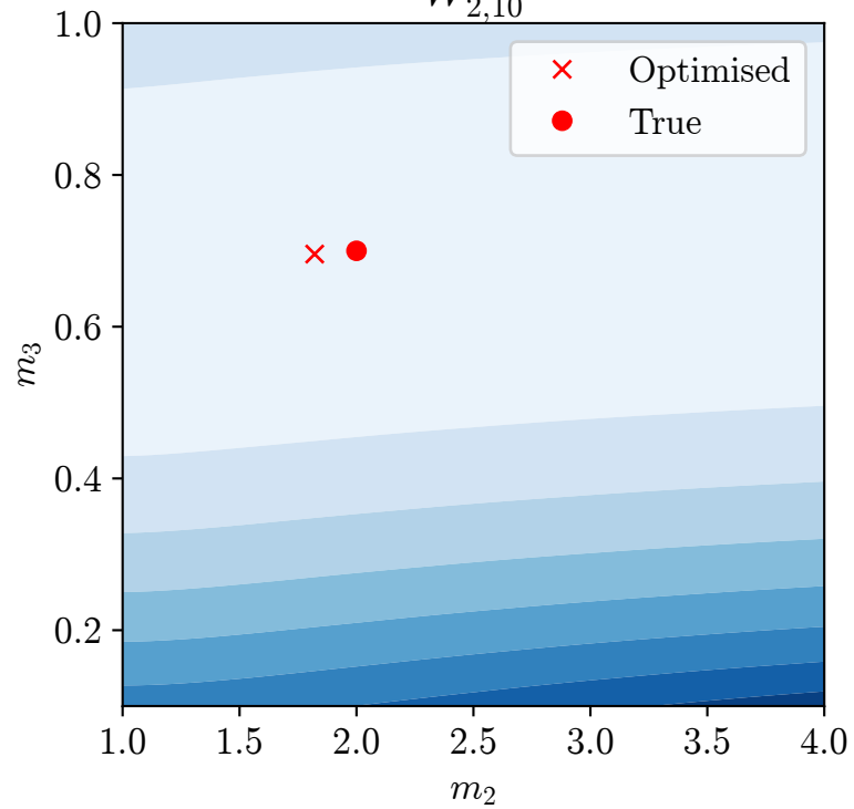
W_{2,10}^2
