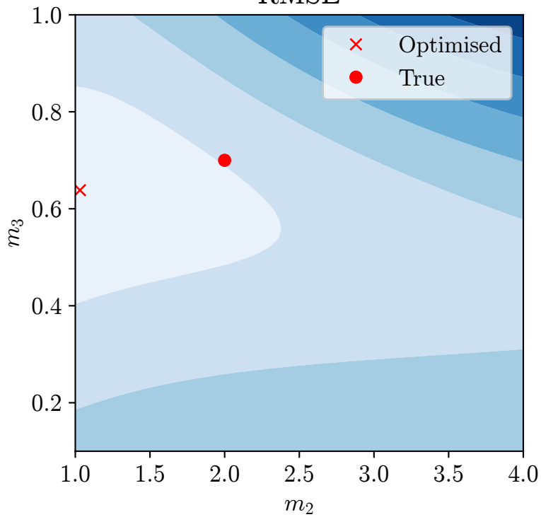
RMSE
