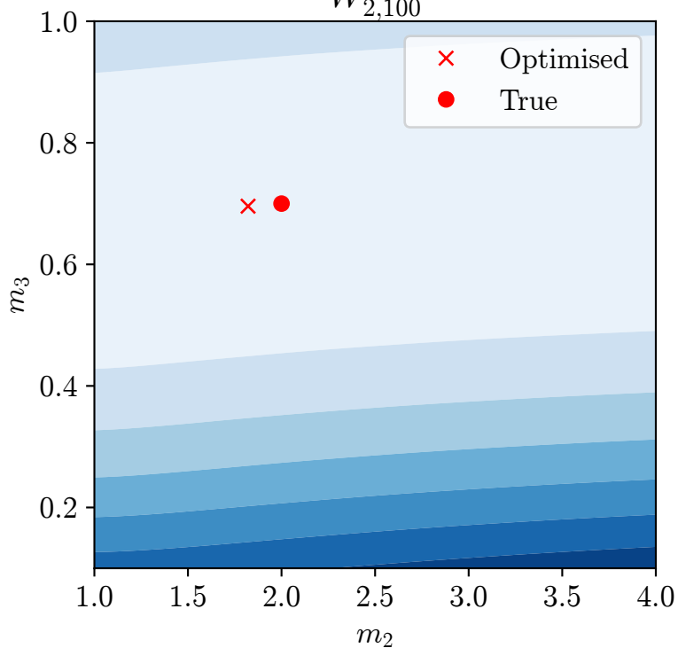
W_{2,100}^2
