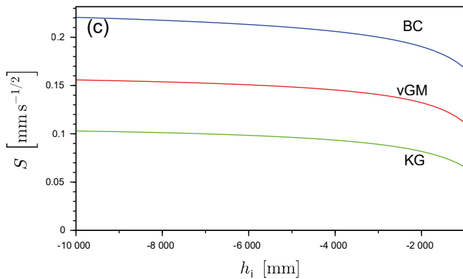
Sorptivity ~ initial water pressure head h_i
