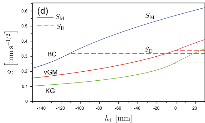
Sorptivity ~ final water pressure head h_f
