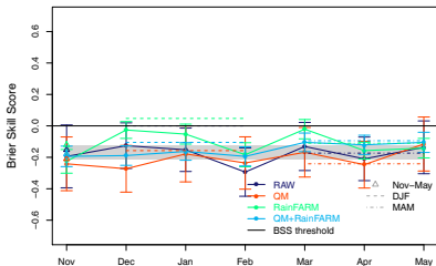
mfS6 BRIER SKILL SCORE Upper Extreme
