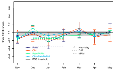
ecmwfS5 BRIER SKILL SCORE Upper Extreme
