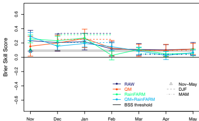
mfS6 BRIER SKILL SCORE Lower Extreme
