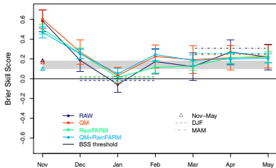
ecmwfS5 BRIER SKILL SCORE Lower Extreme
