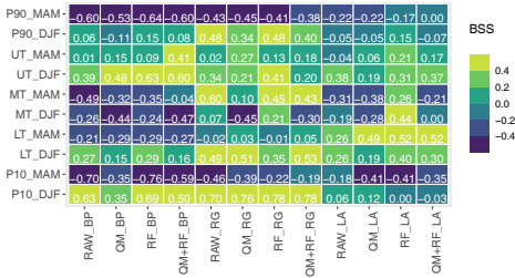
(b) Area under the ROC curve Skill Score MFS6
