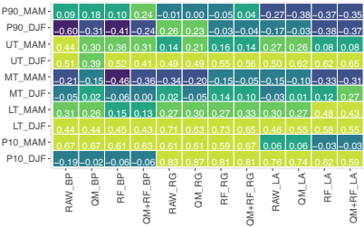
(a) Area under the ROC curve Skill Score ECMWFS5
