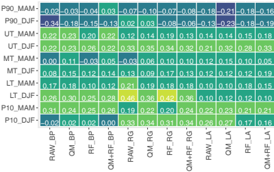
(a) Brier Skill Score ECMWF5
