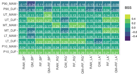
(b) Brier Skill Score MFS6
