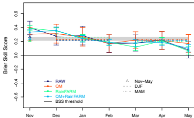
ecmwfS5 BRIER SKILL SCORE Upper Tercile
