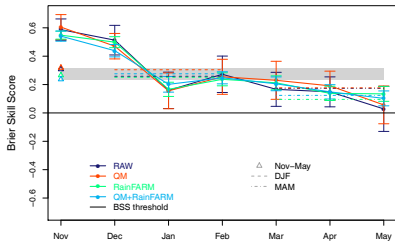
ecmwfS5 BRIER SKILL SCORE Lower Tercile
