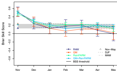
mfs6 BRIER SKILL SCORE Upper Tercile
