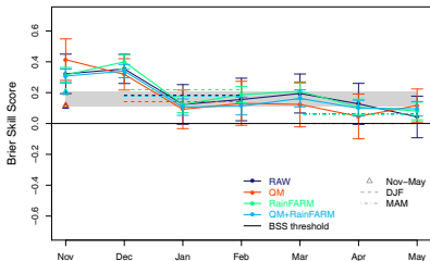
mfs6 BRIER SKILL SCORE Lower Tercile
