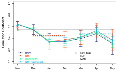
ecmwfS5 FCST-OBS Time Correlation
