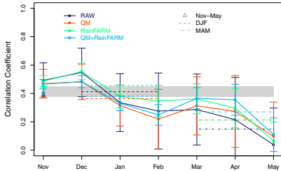
mfS6 FCST-OBS Time Correlation
