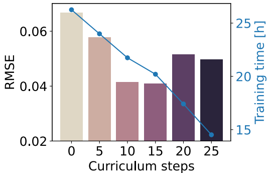
(b) Curriculum learning
