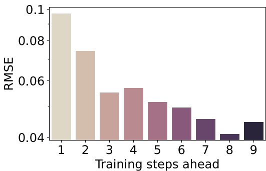
(a) Multi-step-ahead loss
