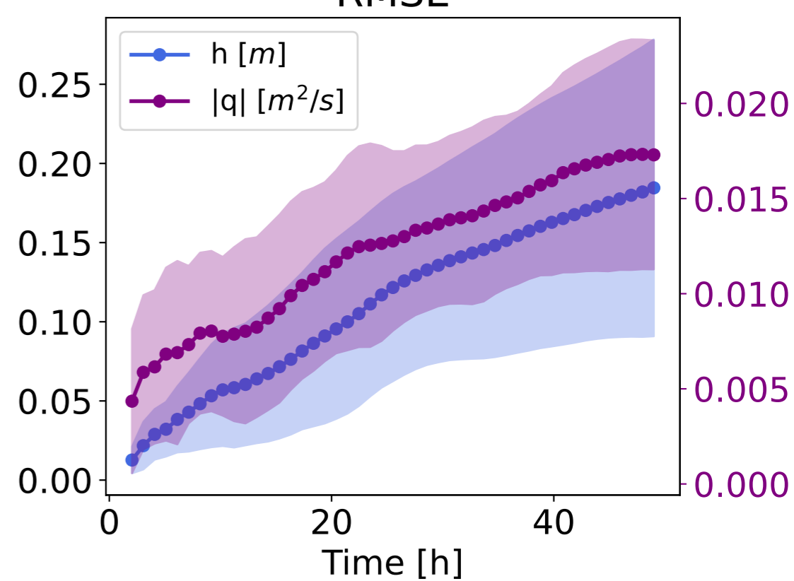
RMSE
