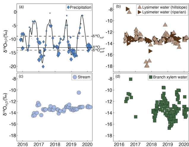
Figure 3. \delta^{18}\text{O} of (a) precipitation, with the size of the marker representing the relative amount of precipitation that fell in the 2 weeks prior to sample collection and the solid line showing a smooth spline fit; (b) lysimeter waters; (c) stream water; and (d) branch xylem water from a tropical montane cloud forested watershed in the southeastern Peruvian Andes mountains.
