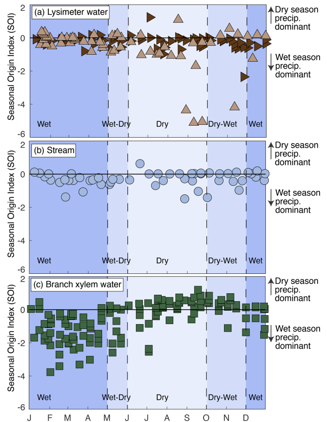
Figure 4. Intra-annual patterns of the seasonal origins of lysimeter, stream, and branch xylem waters from the years 2016 to 2020 in a tropical montane cloud forested watershed in the southeastern Peruvian Andes mountains. Lysimeter water was collected from two lysimeters, one in the stream riparian area (dark-brown sideways-facing triangles) and one on the hillslope (light-brown upwards-facing triangles). The x axis shows months. Blue shading indicates the transitions between seasons.
