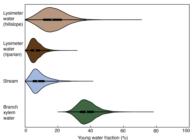
Figure 5. Violin and inset boxplots of the young water fractions ( F_{yw} ) for lysimeter, stream, and branch xylem water, as determined from a bootstrap resampling routine. The F_{yw} interquartile range determined from the bootstrap resampling routine was 12 %–22 % for the hillslope lysimeter water, 4 %–9 % for the riparian water, 5 %–11 % for the stream water, and 34 %–41 % for the branch xylem water. F_{yw} values were calculated using data on isotopic composition of waters from the years 2016 to 2020 in a tropical montane cloud forested watershed in the southeastern Peruvian Andes mountains.
