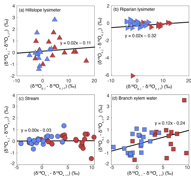
Figure 6. Ensemble hydrograph separation performed on lysimeter waters (a, b), stream waters (c), and tree branch xylem waters (d) in a tropical montane cloud forested watershed in the southeastern Peruvian Andes mountains. The x axis is the \delta^{18}O of precipitation at a given time step minus the stream or xylem \delta^{18}O at the previous time step. The y axis is the stream or xylem \delta^{18}O at a given time step minus the stream or xylem \delta^{18}O at the previous time step. The slopes of the regression line through the stream and branch xylem water datasets are equivalent to their respective new water fractions. Blue symbols indicate stream and branch xylem water samples collected during the wet season, while red symbols indicate samples collected during the dry season. ANCOVA indicated no significant differences between the wet and dry seasons.
