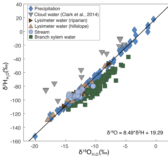
Figure 2. Precipitation, stream, soil, and plant water isotope ratios collected between 2016 and 2020 from a tropical montane cloud forested watershed in the southeastern Peruvian Andes mountains. The regression line and the accompanying equation represent the local meteoric water line. Cloud water isotope ratios are from Clark et al. (2014). Lysimeter water was collected from two lysimeters, one in the stream riparian area (dark-brown sideways-facing triangles) and one on the hillslope (light-brown upwards-facing triangles).
