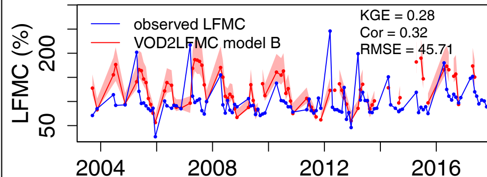
(c) Site with percentile 50% of KGE
