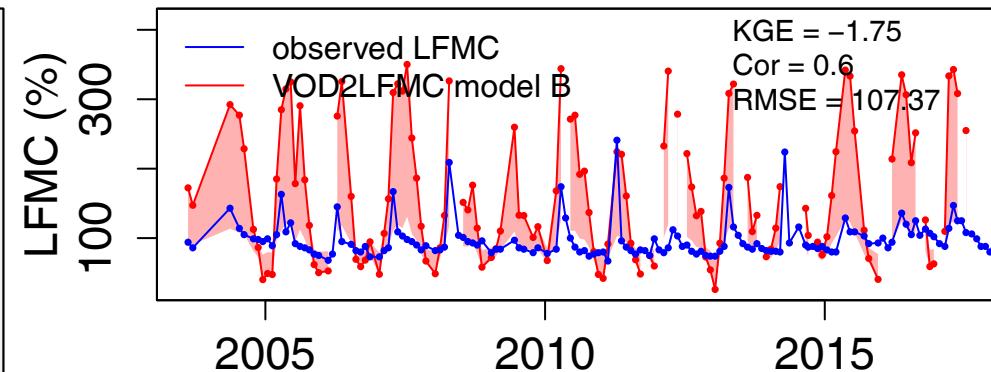
(c) Site with percentile 50% of KGE
