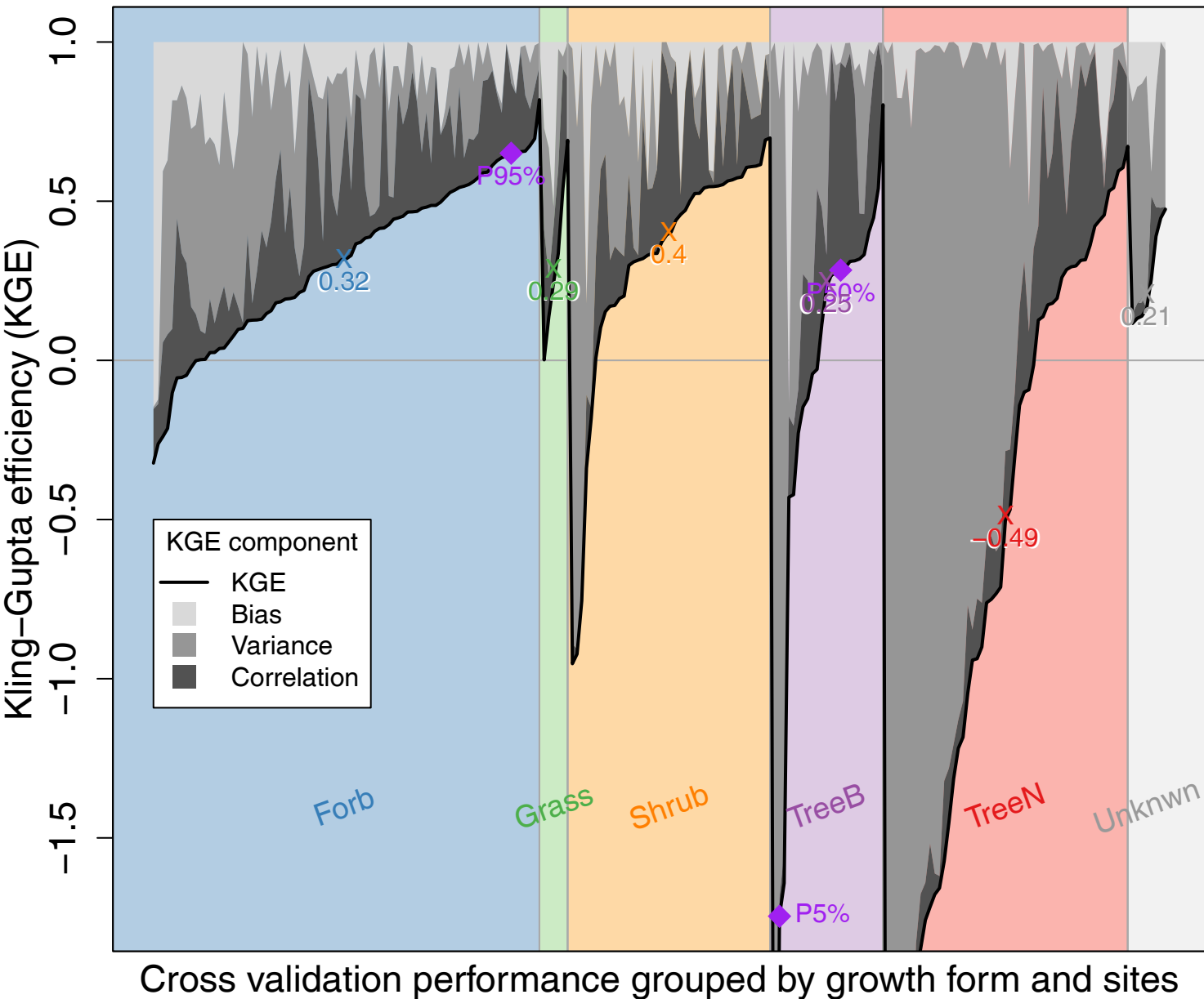
(a) Cross-validation performance model B
