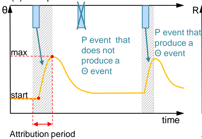
(a) Precipitation and soil moisture events
