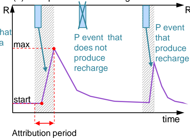
(b) Precipitation and recharge events
