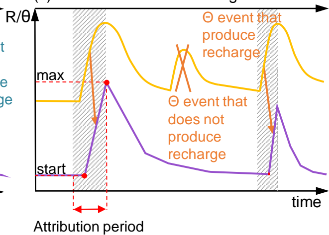
(c) Soil moisture and recharge events
