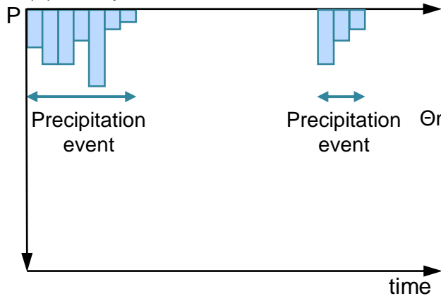
(a) Precipitation events selection
