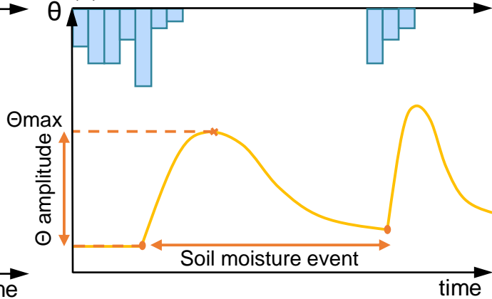
(b) Soil moisture events selection
