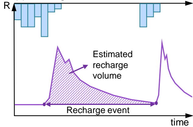
(c) Recharge events selection
