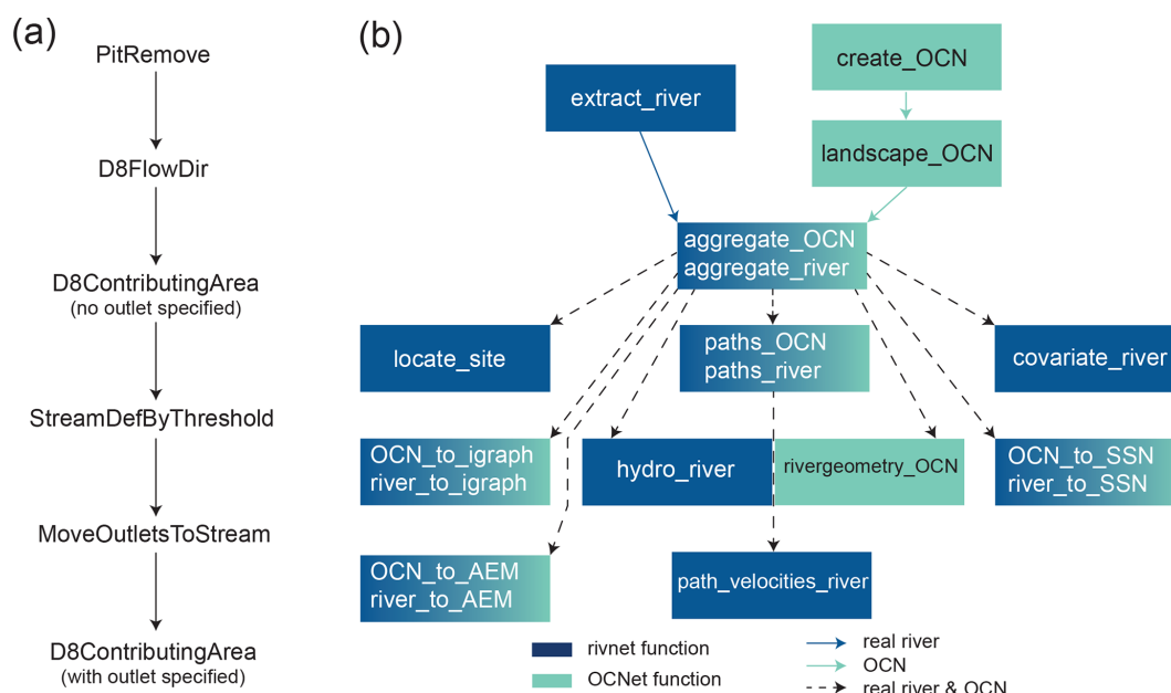
Figure 1. (a) Sequence of TauDEM commands operated by extract_river . (b) Structure of the rivnet and OCNet packages. In both panels, arrows indicate that the output of a function is used as input of the next function.
