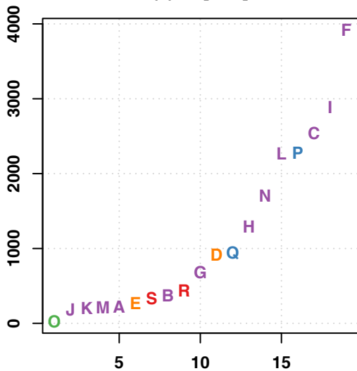
(a) S [km 2 ]
