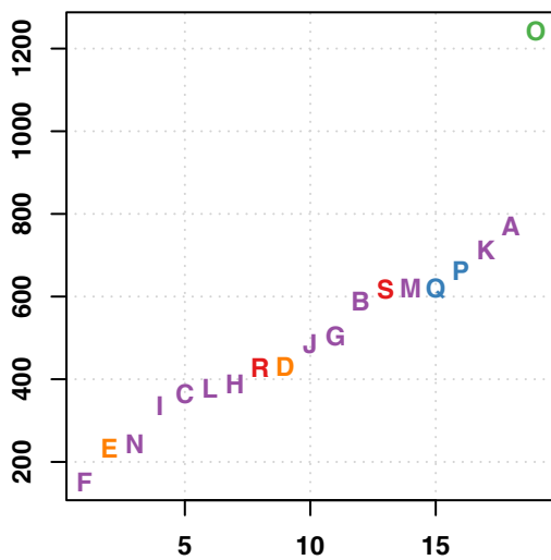
(e) QA [mm/yr]
