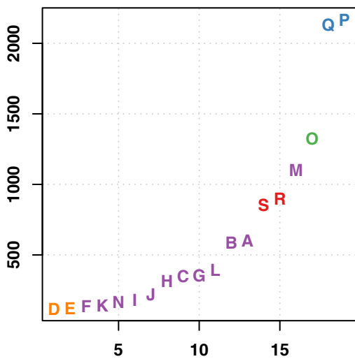
(b) Z50 [m]
