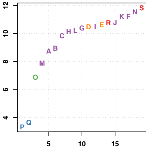
(c) TA [°C]
