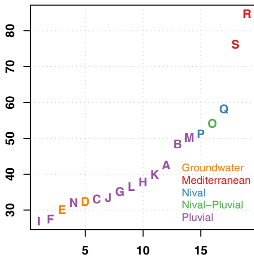
(f) PdMAX [mm/d]
