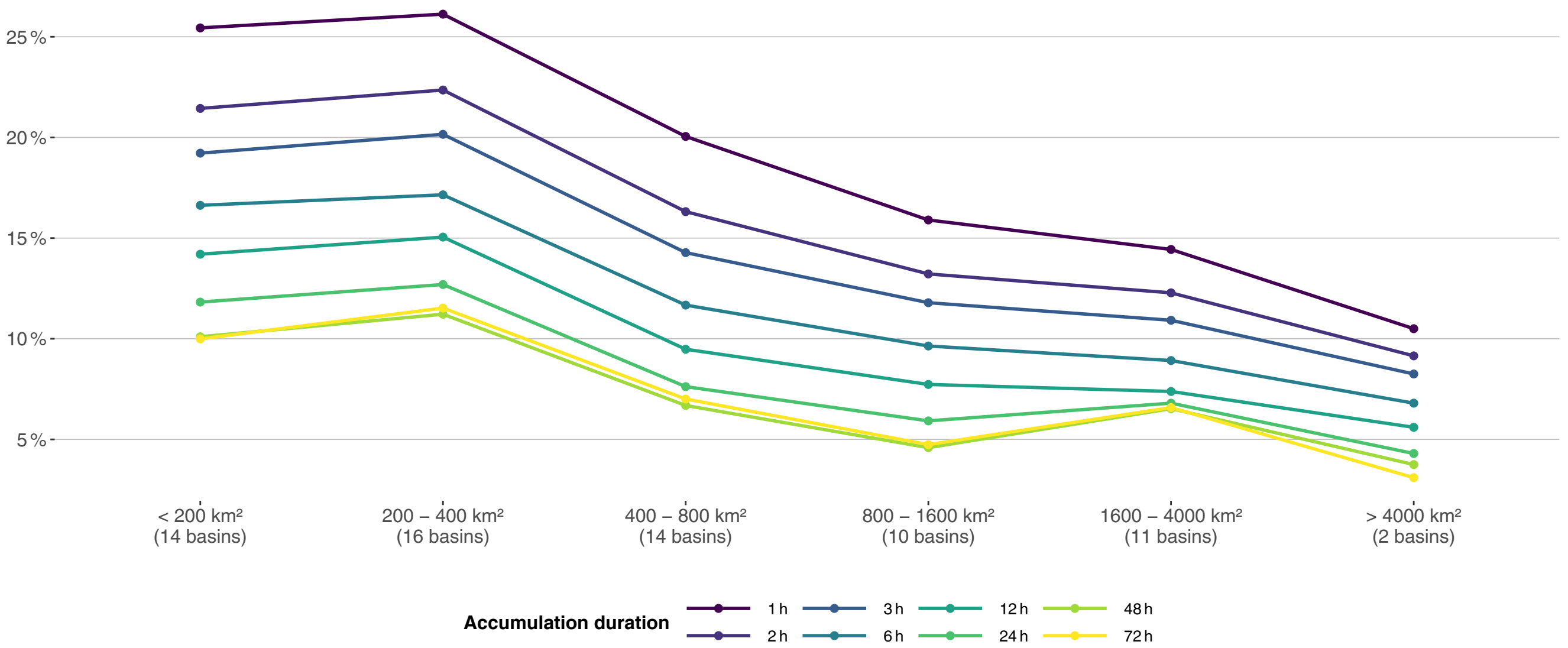
Mean absolute error (MAE) between all IDW and RADFLOOD21 accumulations from 13 July to 16 July 2021 for various durations between 1 and 72 h and for 67 catchments of various sizes
