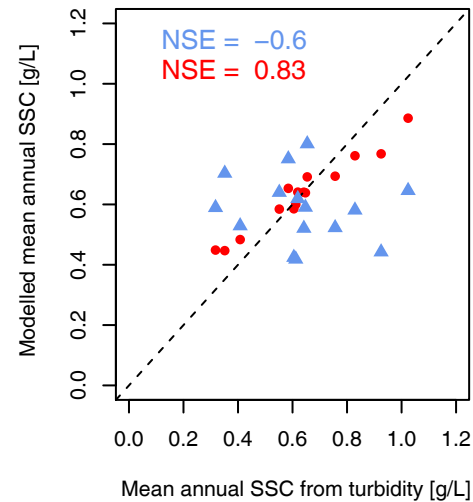
(c) Mean annual SSC
