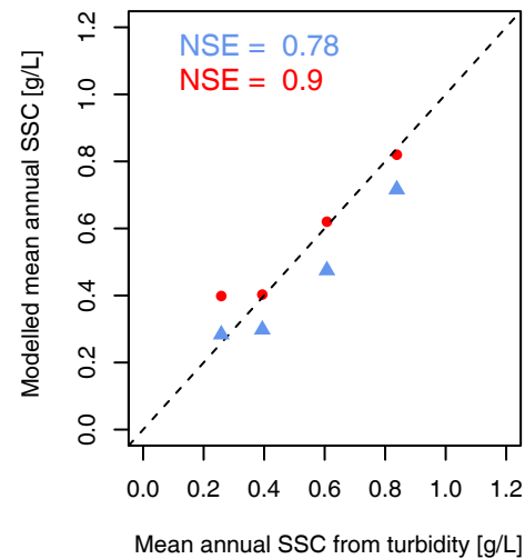
(f) Mean annual SSC
