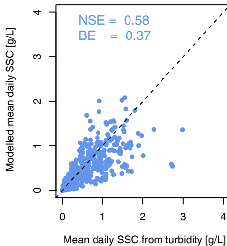
(e) Sediment rating curve
