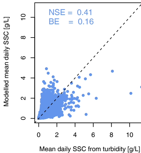
(b) Sediment rating curve
