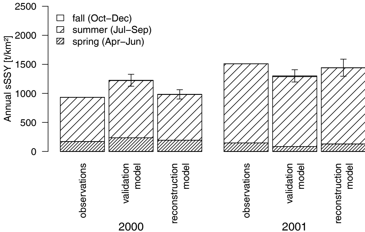
(b) Validation of annual sSSY
