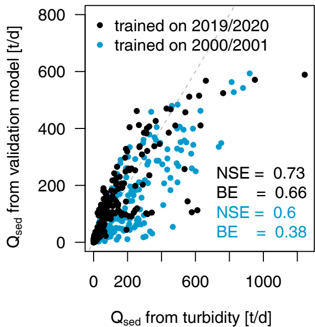
(a) Validation of daily Q_{sed}
